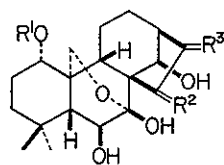
(30) R^1=Ac, R^2=\alpha-H, \beta-OH, R^3=CH_2
