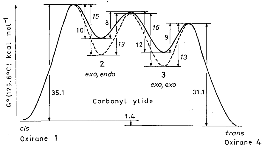
Figure 3. Lower (—) and upper limits (----) for the depths of the energy troughs of the carbonyl ylides 2 and 3 at 129.6°C; the disrotatory ring opening 1 \rightarrow 3 has been omitted for the sake of clarity.
