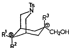
8a R 1 =R 2 =H R 3 =CHO b R 1 =R 2 =OCH 3 R 3 =CHO c R 1 R 2 =-SCH 2 CH 2 S- R 3 =CHO 9a R 1 =R 2 =H R 3 =CH 2 OH b R 1 =R 2 =OCH 3 R 3 =CH 2 OH c R 1 R 2 =-SCH 2 CH 2 S- R 3 =CH 2 OH
