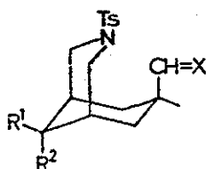
2a R 1 =R 2 =H X=O b R 1 =R 2 =OCH 3 X=O c R 1 R 2 =-SCH 2 CH 2 S- X=O 3a R 1 =R 2 =H X=CH 2 b R 1 =R 2 =OCH 3 X=CH 2
