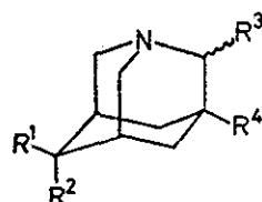
10 R 1 R 2 =O R 3 =OH R 4 =CH 2 OH 11 R 1 R 2 =O R 3 =H R 4 =CHO 12a R 1 =R 2 =H R 3 =H R 4 =CH 2 OH b R 1 R 2 =-SCH 2 CH 2 S- R 3 =H R 4 =CH 2 OH 16 R 1 R 2 =-SCH 2 CH 2 S- R 3 =H R 4 =H
