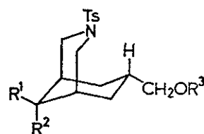
13a R 1 =R 2 =H R 3 =C(=O)CH 3 b R 1 R 2 =-SCH 2 CH 2 S- R 3 =C(=O)CH 3 15 R 1 =R 2 =R 3 =H
