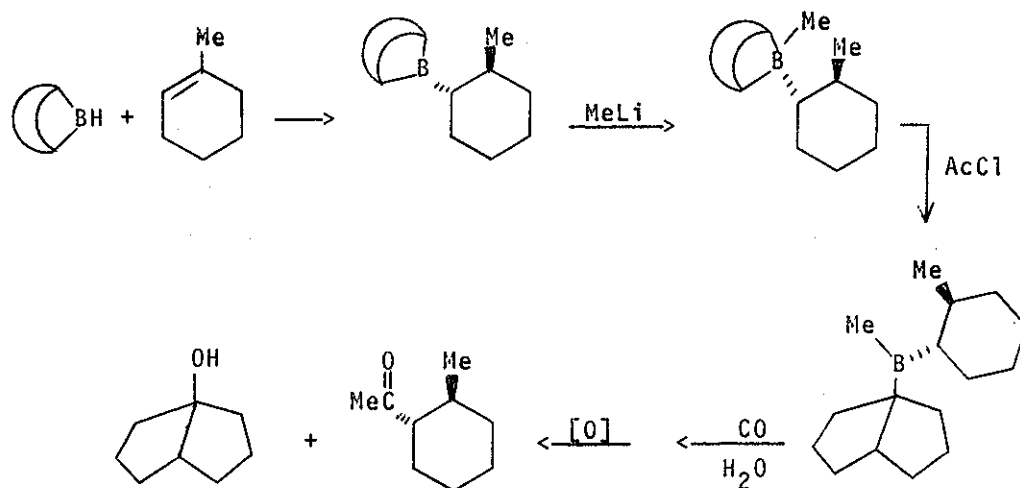
SCHEME III. Synthesis of Mixed Ketones via Butterflyboranes
