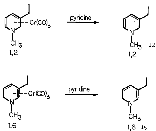
Figure 11. The synthesis of N-methyl-3-ethyl-1,2-dihydropyridine (12) and N-methyl-3-ethyl-1,6-dihydropyridine (15) from the chromium complexes.
