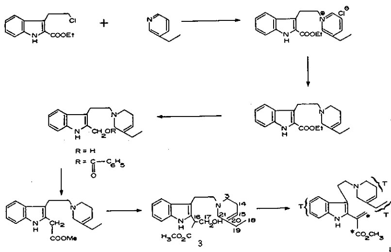
Figure 3. Synthesis of 16,17-dihydrosecodin-17-ol (3) and secodine (4).
