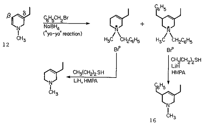
Figure 12. Alkylation studies with N-methyl-3-ethyl-1,2-dihydropyridine (12).
