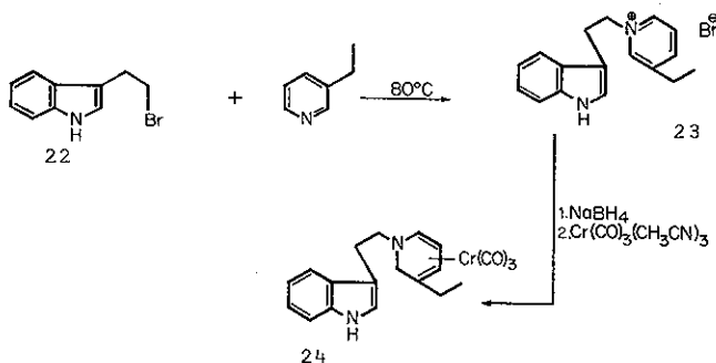
Figure 16. The synthesis of the chromium carbonyl complex 24.
