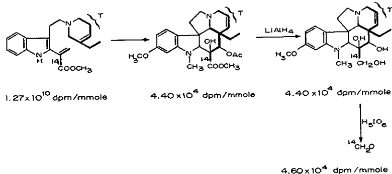
Figure 4. Degradation of vindoline from [ 14 C 14 COOCH 3 ,3,14,15,21- 3 H]-secodine.
