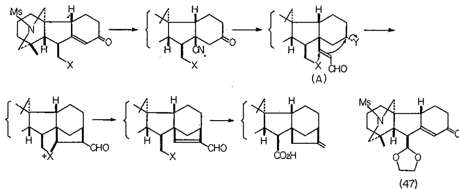
Scheme 16
