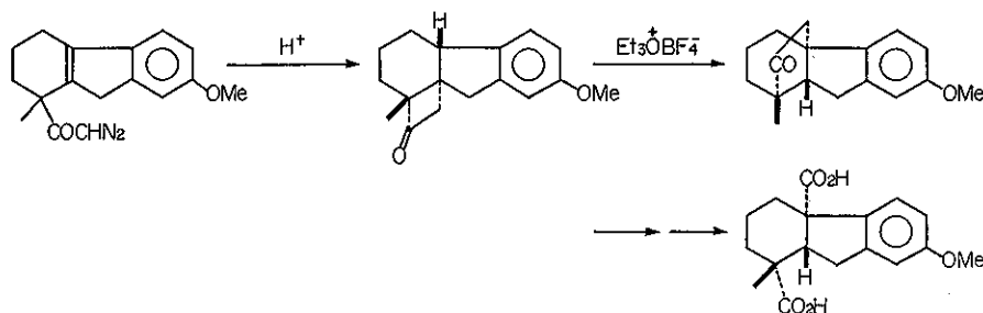
Scheme 37
