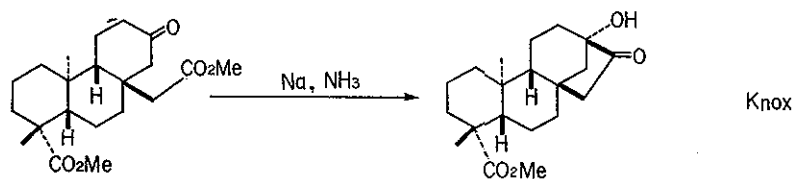
Scheme 34
