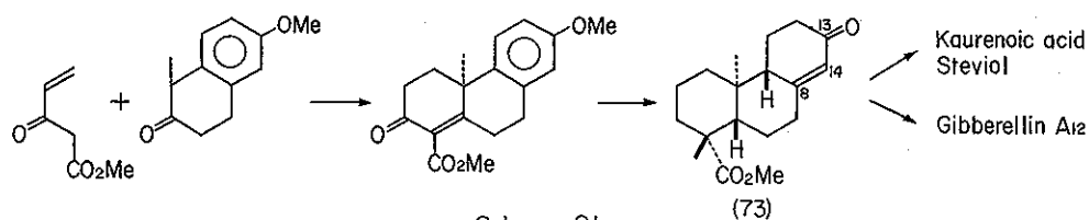
Scheme 21
