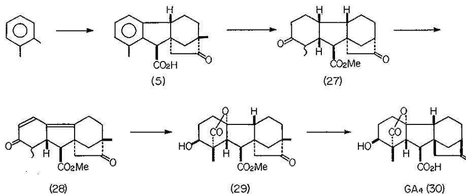
Scheme 9
