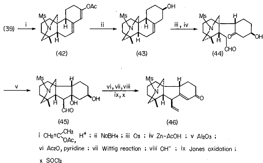
Scheme 15
