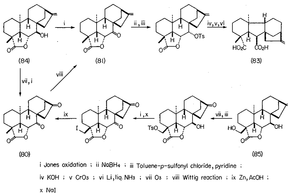
Scheme 23
