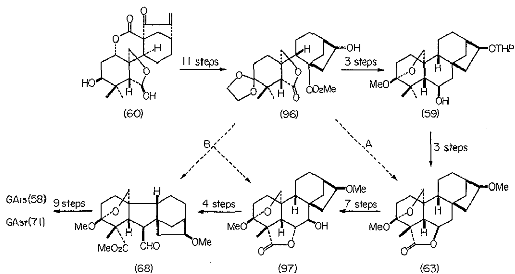
Scheme 25
