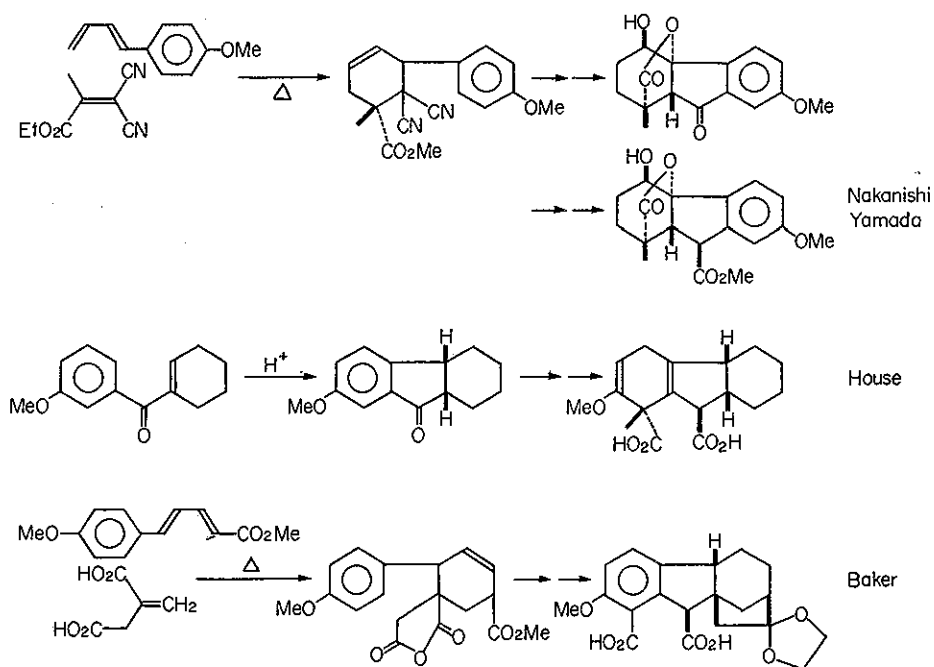
Scheme 36
