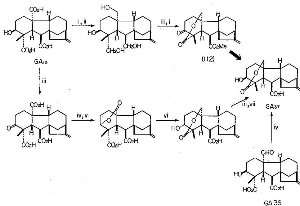
Scheme 31
