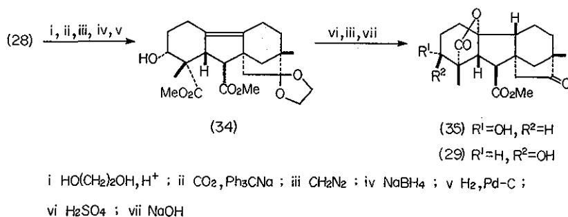
Scheme 12
