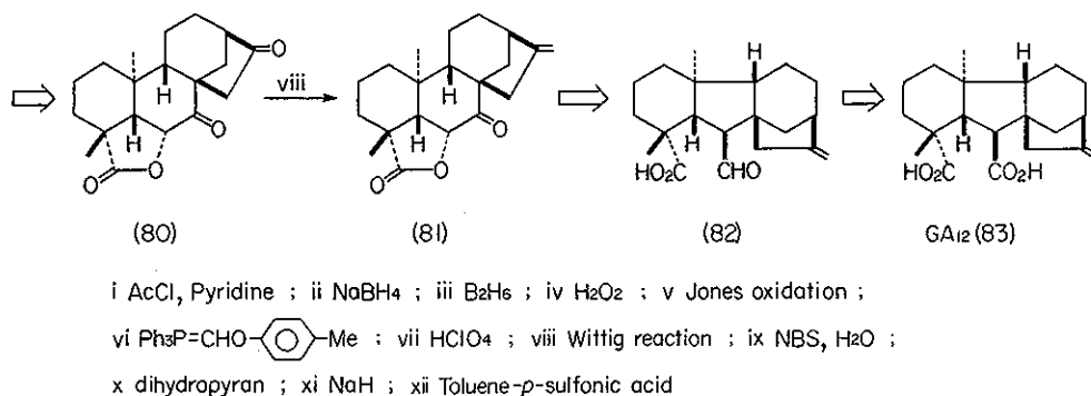
Scheme 22
