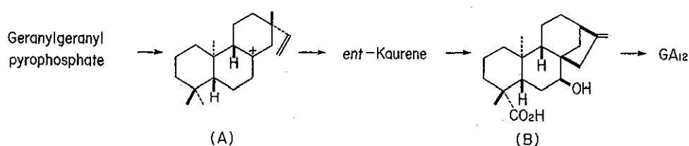
Scheme 20
