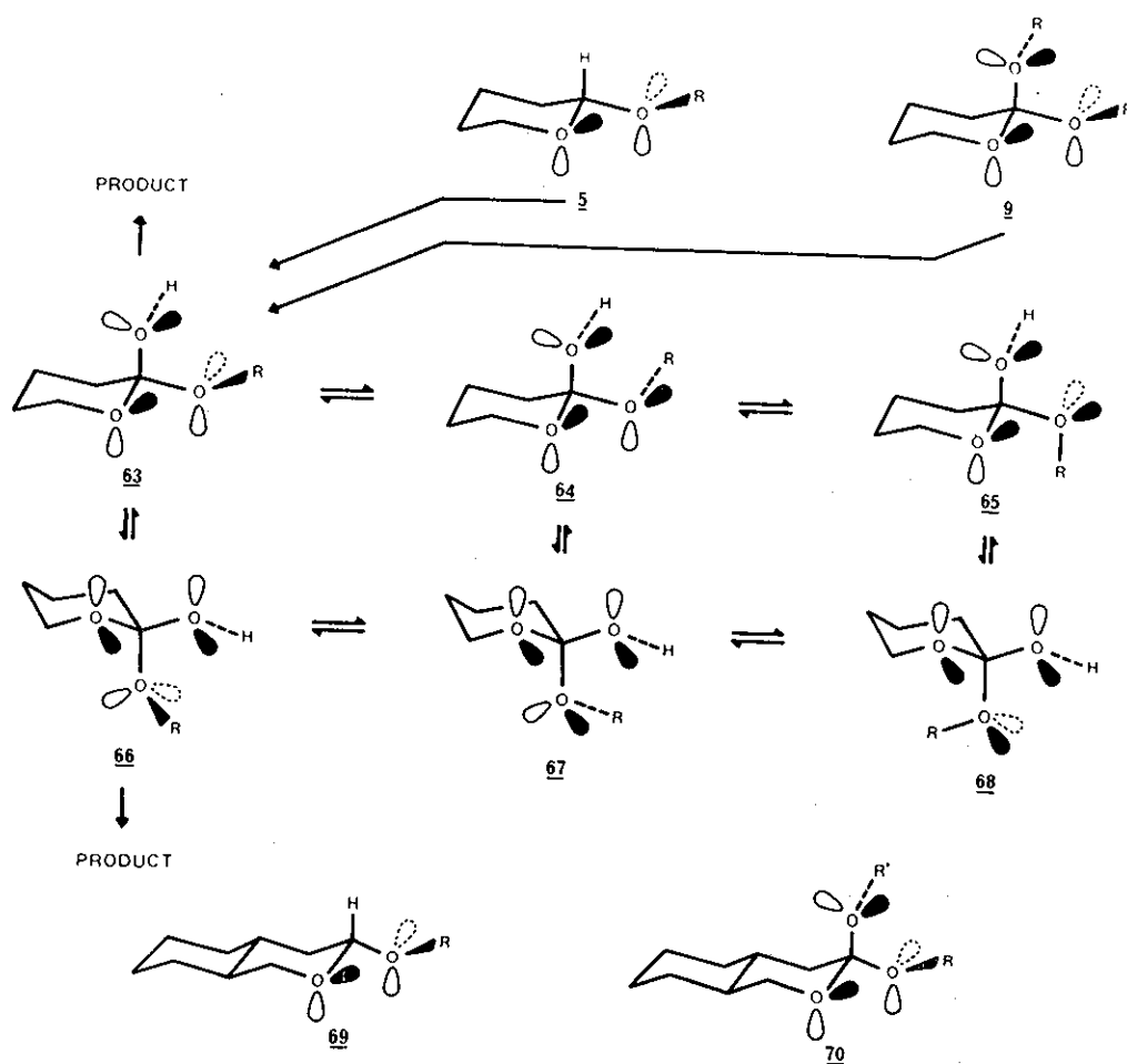
SCHEME 13
