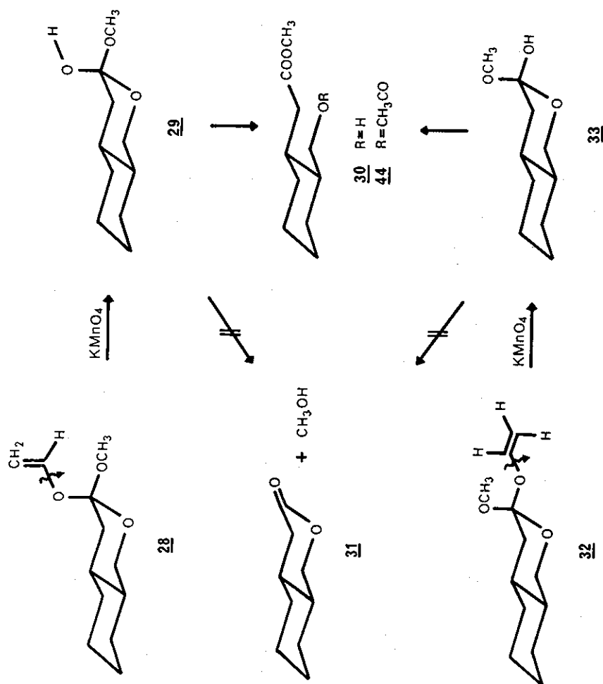
SCHEME 8
