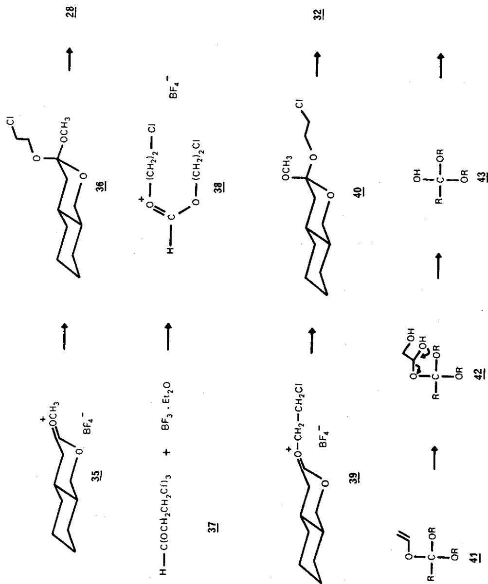
SCHEME 9
