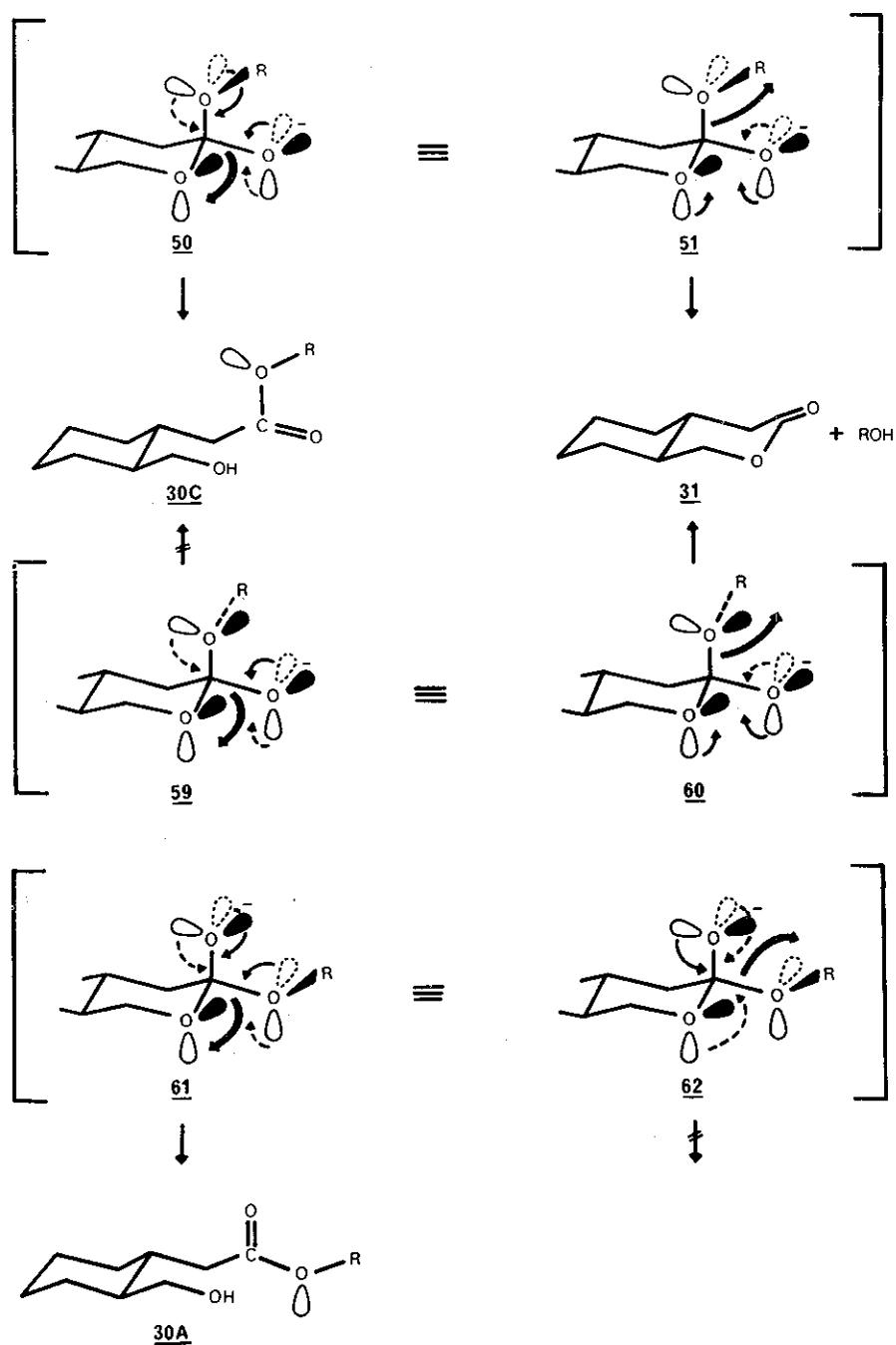
SCHEME 11
