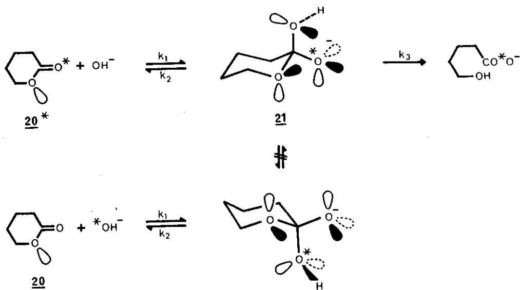
SCHEME 5 (O* = O 18 )
