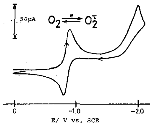
Fig. 1. Cyclic voltammograms of oxygen. electrolyte: 0.1 M TEAP/ DMF, electrode: HMDE, sweep rate: 0.1 Vs -1 .
