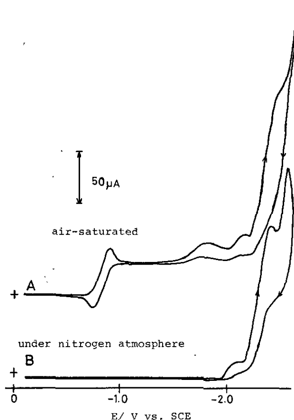
Fig. 4. Cyclic voltammograms of the catholyte in the presence of 4-methylpyridine-N-oxide. electrolyte: 0.1 M TEAP/ DMF, electrode: HMDE.
