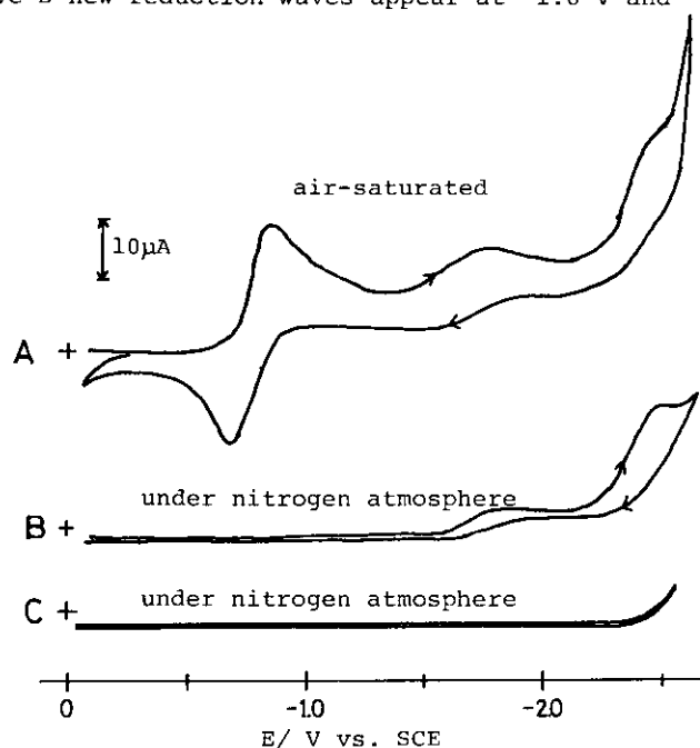
Fig. 3. Cyclic voltammograms of the catholyte in the presence of 4-methylpyridine. electrode: HMDE, electrolyte: 0.1 M TEAP/ DMF.
