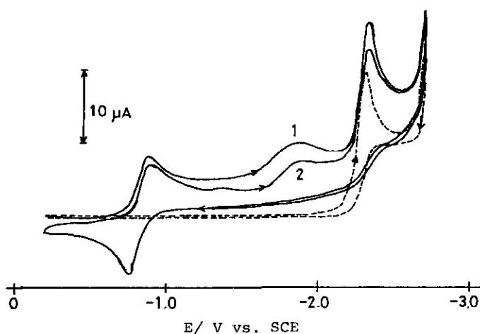
Fig. 2. Cyclic voltammograms of 4-methylpyridine-N-oxide in the presence ( — ) and in the absence ( --- ) of oxygen. electrolyte: 0.1 M TEAP/ DMF, electrode: HMDE, sweep rate: 0.1 \text{ Vs}^{-1} , 1: the first sweep, 2: the second sweep.
