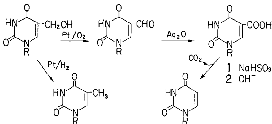
Fig. 8 Interconversion among the polyoxin nucleosides.
