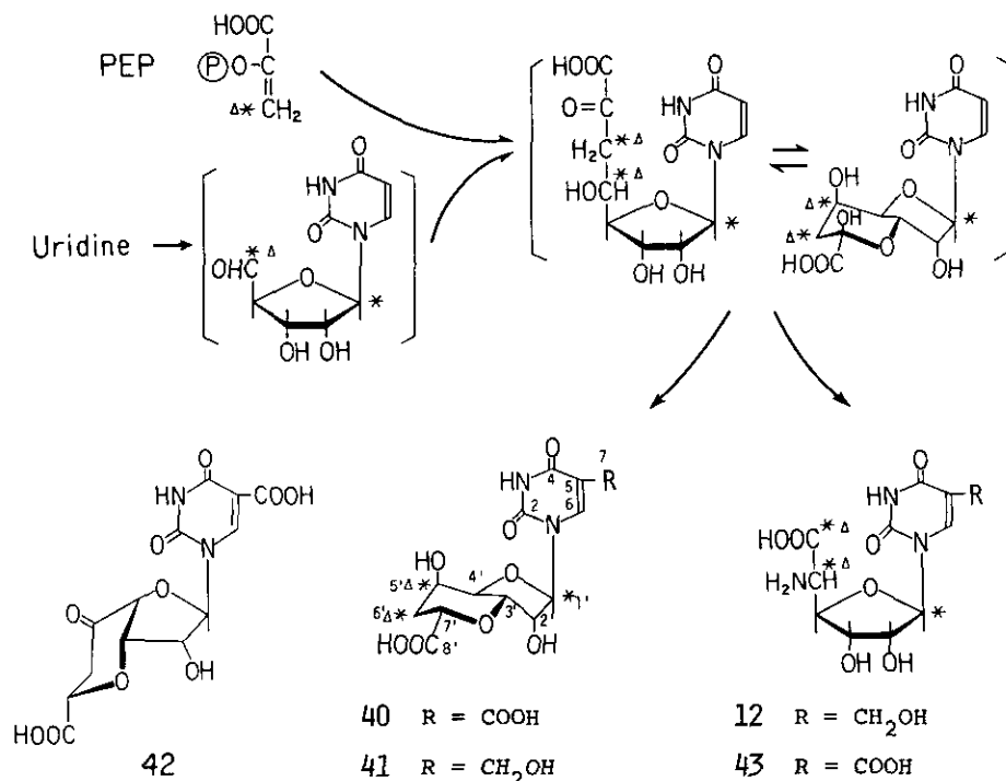
Fig. 11 Biosynthesis of the nucleoside skeleton of the polyoxins and octosyl acids. * Label from [1-^{13}\text{C}] glucose, \Delta from [6-^{13}\text{C}] glucose. Incorporation stage of the one-carbon unit is not known.
