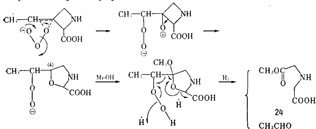
Fig. 6 Ozonolysis of polyoximic acid.
