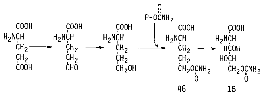
Fig. 13 Biosynthetic pathway for carbamoylpolyoxamic acid.
