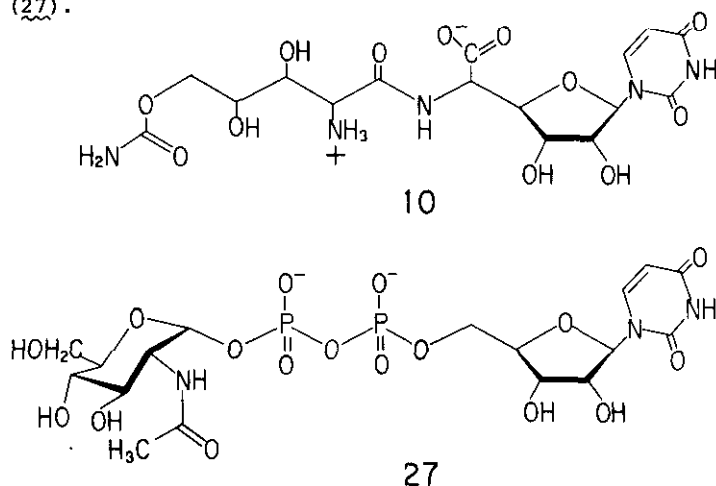
Fig. 9 Structural similarity of polyoxin L (10) and UDP-N-acetylglucosamine (27).
