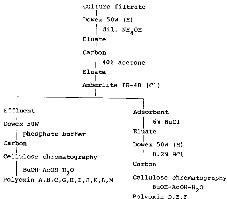
Fig.1 Isolation procedure for polyoxins.
