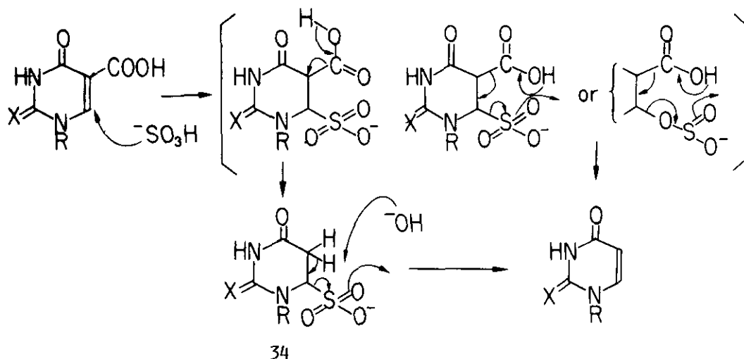
Fig. 10 Bisulfite-catalysed decarboxylation of 5-carboxyuracils.
