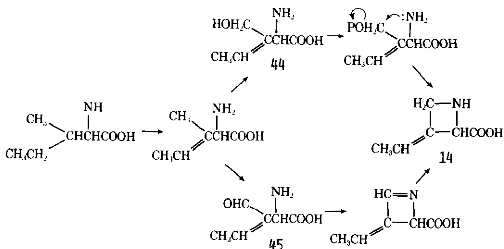
Fig. 12. Proposed biosynthetic pathway for polyoximic acid.
