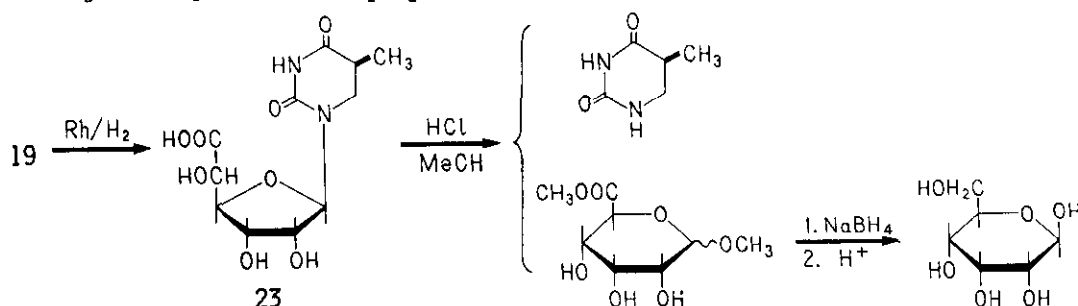
Fig. 5 Degradation of polyoxin C.
