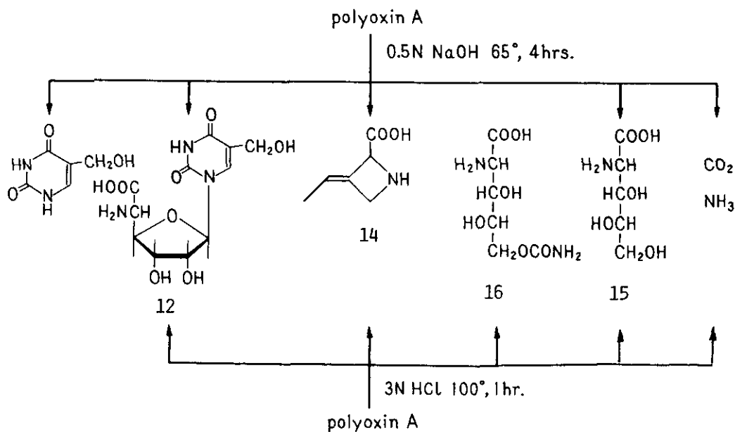
Fig. 3. Hydrolysis of polyoxin A
