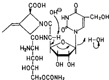
Fig. 7. Alkaline hydrolysis mechanism of polyoxin A.
