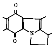
mitosene type
