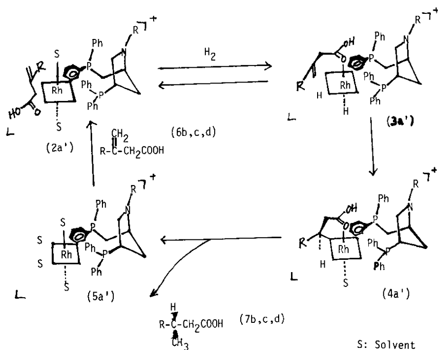
Fig. 3. (B) Mechanism for \beta -Methylene Acids ( Bifunctional Acids )
