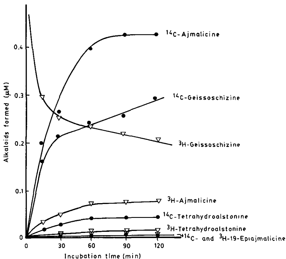
FIGURE 1. Incorporation of geissoschizine and tryptamine into ajmalicine and isomers. Incubations were carried out with a mixture of 2 \mu\text{Ci} [ 2\text{-}^{14}\text{C} ]-tryptamine (4.0 \mu\text{M} ) and 15 \mu\text{Ci} [aryl- ^3\text{H} ]-geissoschizine (2.0 \mu\text{M} ) at 37^\circ\text{C} in 0.05 M citrate buffered solution (pH 7.2) containing 10 mM mercaptoethanol, 20 mM NADP, and 4.0 \mu\text{M} secologanin. Alkaloids were isolated at intervals and purified by tlc systems ( \text{CHCl}_3/\text{MeOH} , 85:15; hexane/acetone/diethylamine, 7:2:1; \text{CHCl}_3/\text{acetone}/\text{hexane} , 5:4:8). Ajmalicine and geissoschizine in each case were recrystallized repeatedly (minimum 4 times) to constant specific activity with the authentic compounds.
