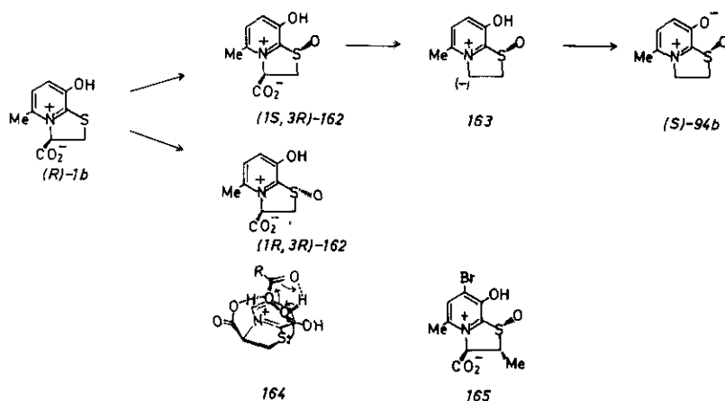
Scheme 29
