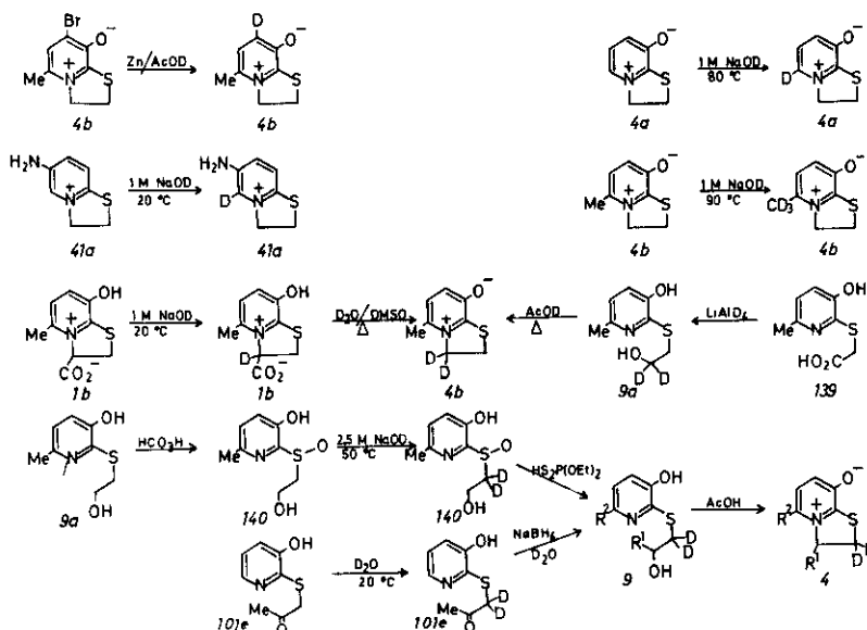
Scheme 26
