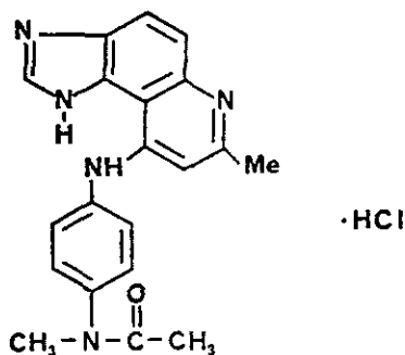
Acodazole Hydrochloride
