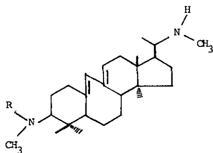
Papilamine (1): R=H
