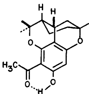
3 Desbenzylidene rubranine
