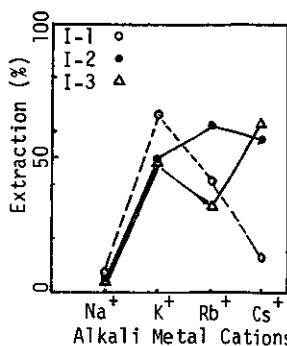
Fig 1 Solvent Extraction of I
