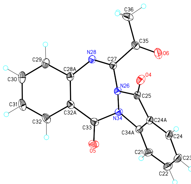
Figure 1b. Molecular structure of 10a , molecule II with ADPs displayed at the 50 % level. The torsion angle N28-C27-N26-N34 is 61.9 ° and the intramolecular, non-bonding O4...O6 distance is 2.907 Å.
