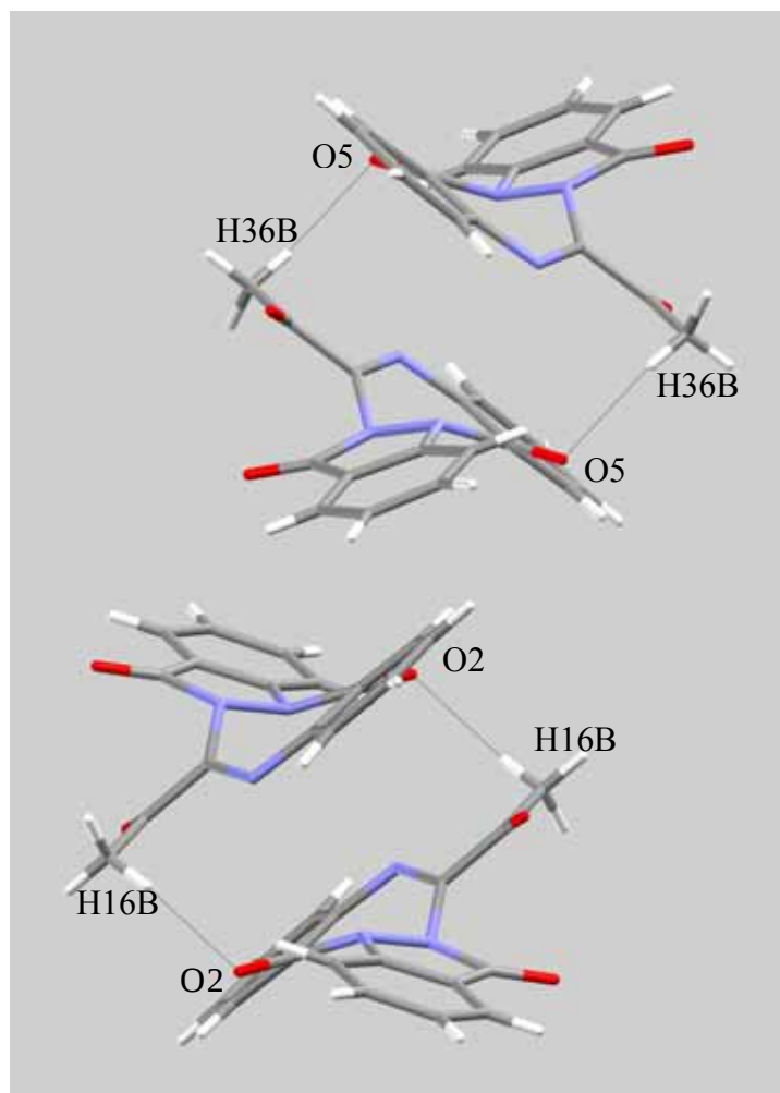
Figure 2. Crystal packing of 10a , viewing down [011]. The racemic pairs of molecules I (upper pair) and of molecules II (bottom pair) are displayed with the intermolecular C-H...O hydrogen bonds at distances of 2.34 Å.
