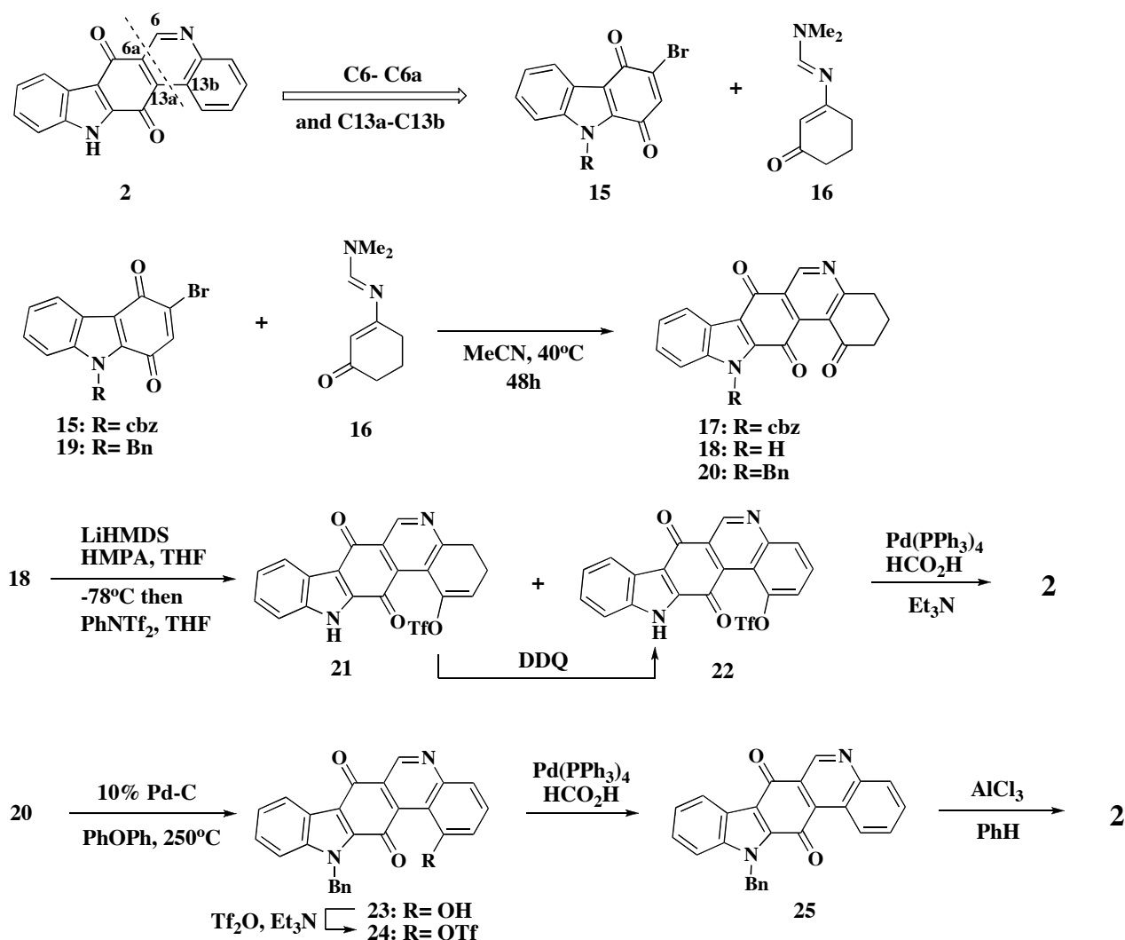
Scheme 3
