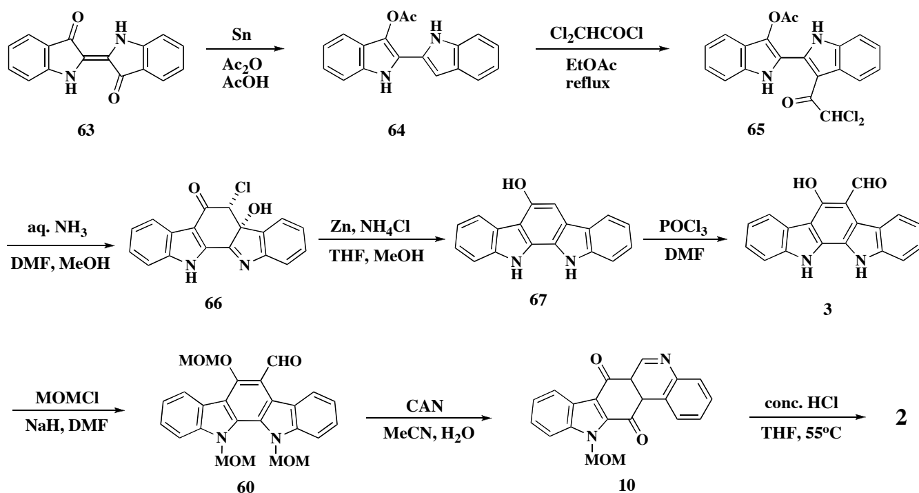
Scheme 9
