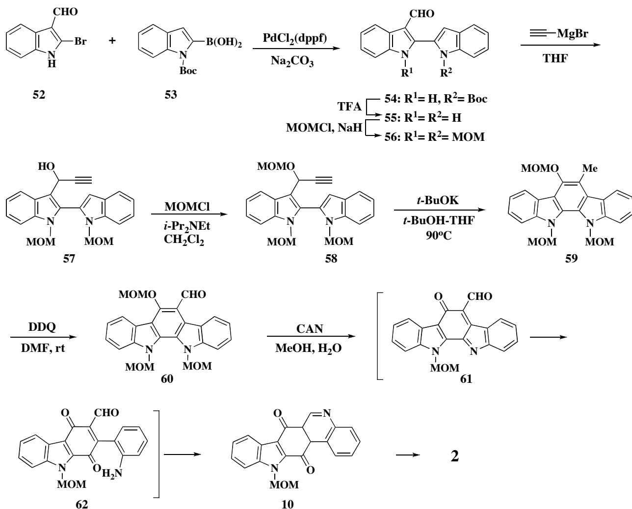
Scheme 8
