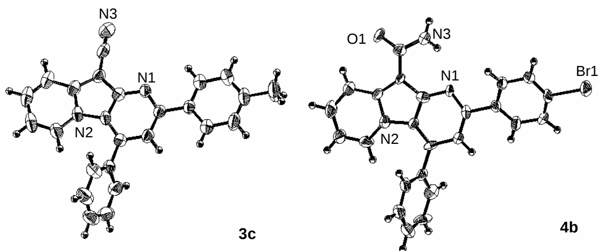
Figure 1. ORTEP drawings of compounds 3c and 4b .
