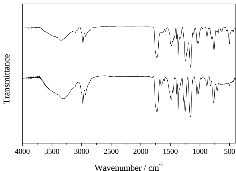
Figure 4. IR spectra of 5(Fe) (top) and 5(Ni) (bottom).
