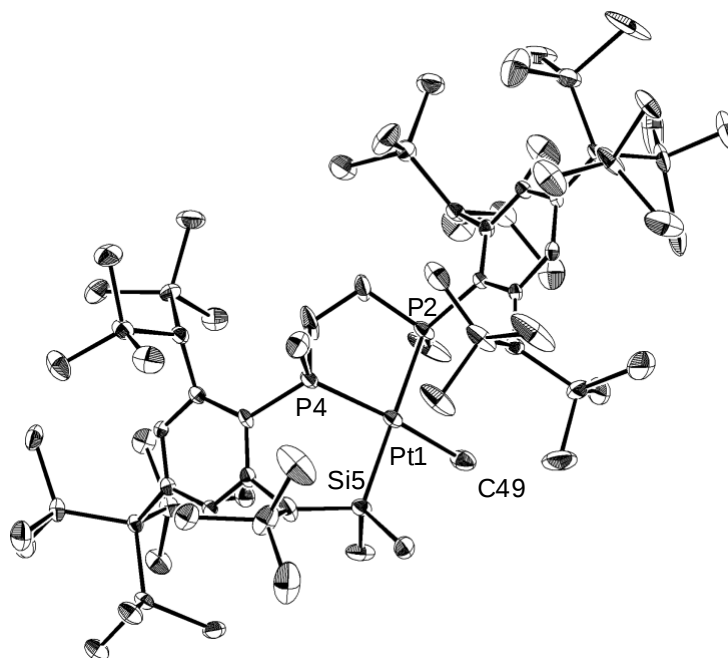
Figure 1. Molecular structure of 4 . Displacement ellipsoids were drawn at the 30% probability level. Selected bond lengths (Å) and angles (°): Pt1-C49 2.118(8), Pt1-Si5 2.3212(18), Pt1-P4 2.275(4), Pt1-P2 2.4190(17), P2-Pt1-P4 88.38(6), P4-Pt1-Si5 93.63(7), Si5-Pt1-C49 83.6(2), C49-Pt1-P2 92.6(2).
