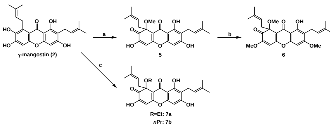
Scheme 2. Reagents and conditions: (a) C.C.E. (0.3 mA/cm 2 ), 2 F/mol, MeOH, 51%. (b) MeI, K 2 CO 3 , DMF, 66%. (c) Oxidized iodobenzene, EtOH or n PrOH, 7a ; 36%, 7b ; 41%.
