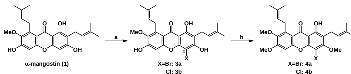
Scheme 1. Reagents and conditions: (a) NBS or NCS, THF, 3a ; 51%, 3b ; 46% (b) MeI, K 2 CO 3 , DMF, 4a ; 67%, 4b ; 77%
