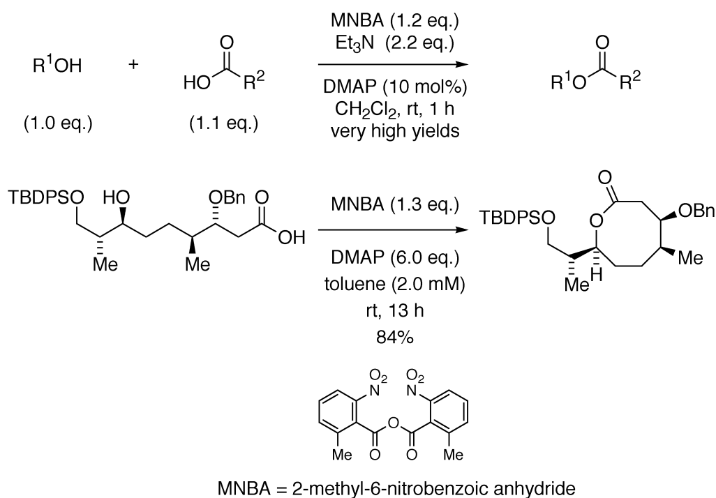
Scheme 1. Effective Synthesis of Carboxylic Esters and Lactones Using MNBA
