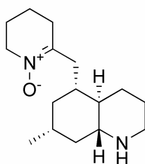
lycposerramine-X ( 39 ) 51 C 16 H 28 N 2 O
