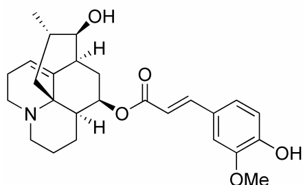
lannotinidine D ( 20 ) 43 \text{C}_{26}\text{H}_{33}\text{NO}_5
