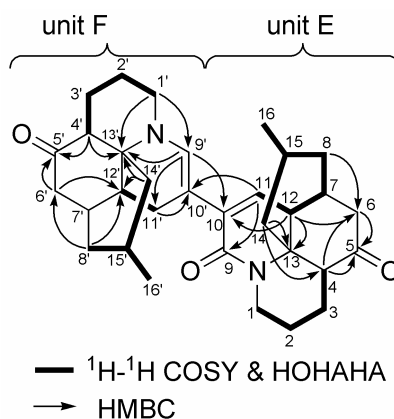
Figure 22. Selected 2D NMR correlations for complanadine C ( 50 ).
