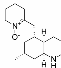
lycoposerramine-Z ( 41 )
