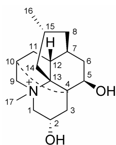
lycopodatine A ( 8 )
