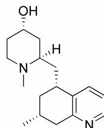
lycposerramine-W ( 38 ) 50 C 17 H 26 N 2 O
