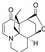
lannotinidine F ( 22 )
