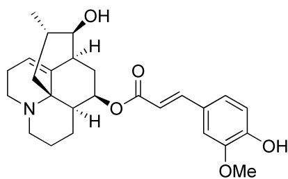
lannotinidine D ( 20 )
