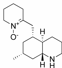
lycoposerramine-X ( 39 )
