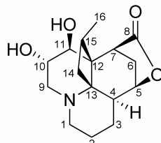
lannotinidine E ( 21 )
