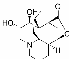
lannotinidine E ( 21 ) 43 \text{C}_{16}\text{H}_{23}\text{NO}_4
