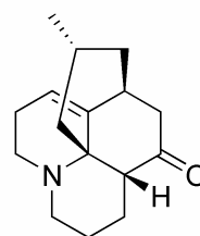
lycopodatine C ( 10 )
