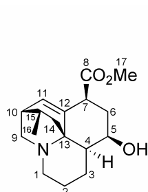
lannotinidine A ( 17 )
