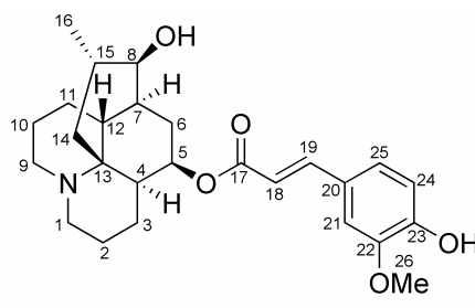
lannotinidine C ( 19 )
