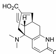
lycoparin A ( 31 ) 48 \text{C}_{17}\text{H}_{20}\text{N}_2\text{O}_3
