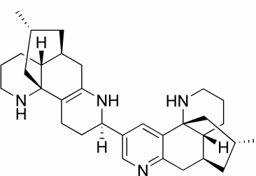
complanadine D ( 51 )
