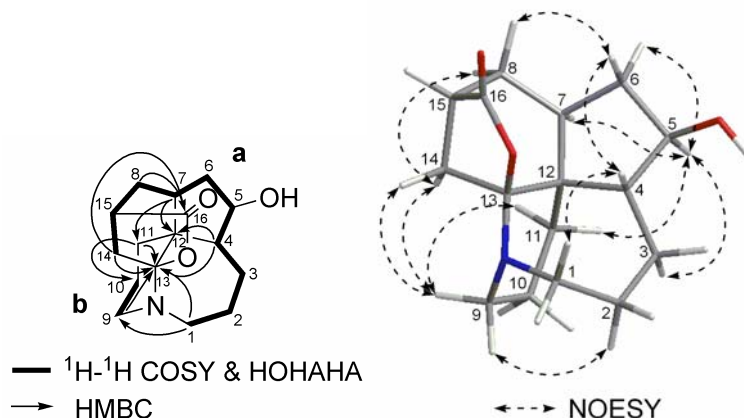
Figure 9. Selected 2D NMR correlations for lycopladiene D ( 27 ).
