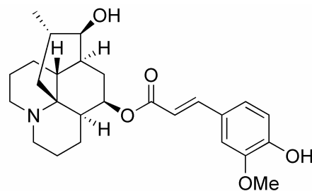
lannotinidine C ( 19 ) 43 \text{C}_{26}\text{H}_{35}\text{NO}_5
