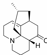
lycopodatine C ( 10 )
