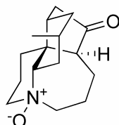
lannotinidine B ( 18 ) 43 \text{C}_{16}\text{H}_{25}\text{NO}_2
