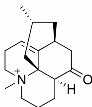
lycopodatine B ( 9 )
