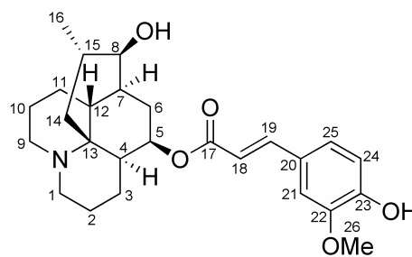
lannotinidine C ( 19 )
