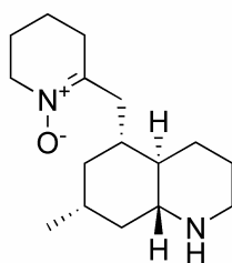
lycoposerramine-X ( 39 )
