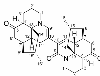
complanadine C ( 50 )
