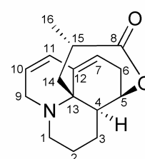
lannotinidine G ( 23 )
