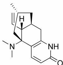
8,15-dihydrohuperzine ( 30 ) 47 \text{C}_{17}\text{H}_{24}\text{N}_2\text{O}
