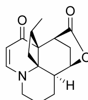
lannotinidine F ( 22 ) 43 \text{C}_{16}\text{H}_{19}\text{NO}_3
