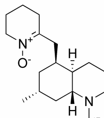
lycoposerramine-Y ( 40 )
