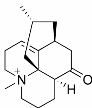
lycopodatine B ( 9 )
