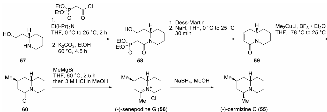
Scheme 1. Synthesis of cermizine C ( 55 ) and senepodine G ( 56 ).
