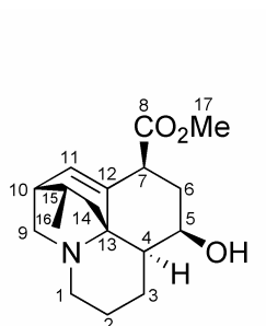
lannotinidine A ( 17 )
