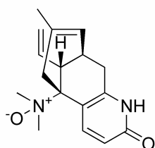
huperzine N-oxide ( 29 ) 47 \text{C}_{17}\text{H}_{22}\text{N}_2\text{O}_2
