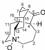
lannotinidine B ( 18 )
