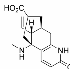
lycoparin B ( 32 ) 48 \text{C}_{16}\text{H}_{18}\text{N}_2\text{O}_3
