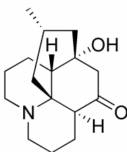
7-hydroxylycopodine ( 3 )
