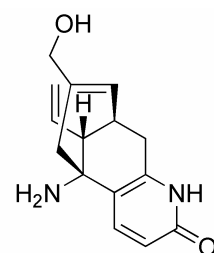
lycoparin C ( 33 ) 48 \text{C}_{15}\text{H}_{18}\text{N}_2\text{O}_2
