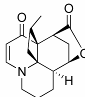
lannotinidine F ( 22 )
