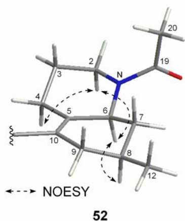
Figure 17. Selected NOESY correlations and relative configurations for an octahydroquinoline ring of tetrahydrodeoxylycoperine A ( 52 ).
