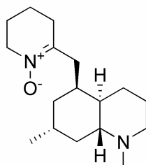
lycposerramine-Y ( 40 ) 51 C 17 H 30 N 2 O
