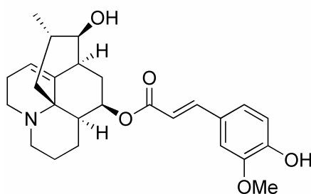
lannotinidine D ( 20 )
