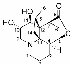
lannotinidine E ( 21 )
