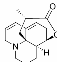
lannotinidine G ( 23 ) 43 \text{C}_{16}\text{H}_{21}\text{NO}_2
