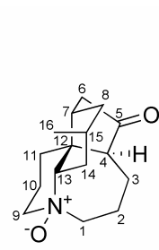
lannotinidine B ( 18 )
