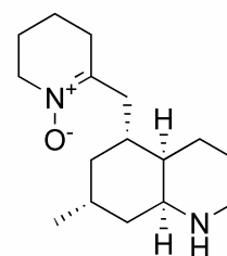
lycposerramine-Z ( 41 ) 51 C 16 H 28 N 2 O
