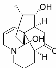
8 \alpha -hydroxylycothunine ( 15 )
