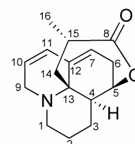
lannotinidine G ( 23 )
