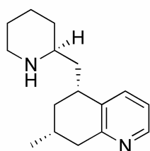
lycposerramine-V ( 37 ) 50 C 16 H 24 N 2
