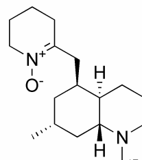
lycoposerramine-Y ( 40 )
