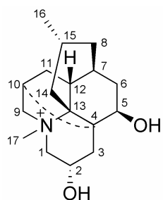
lycopodatine A ( 8 )
