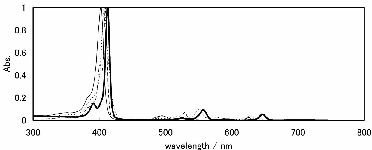
Figure 3. UV-vis spectra of 3 (solid line), 4 (dotted line), 5 (broken line), and 6 (bold line) in CHCl 3 .
