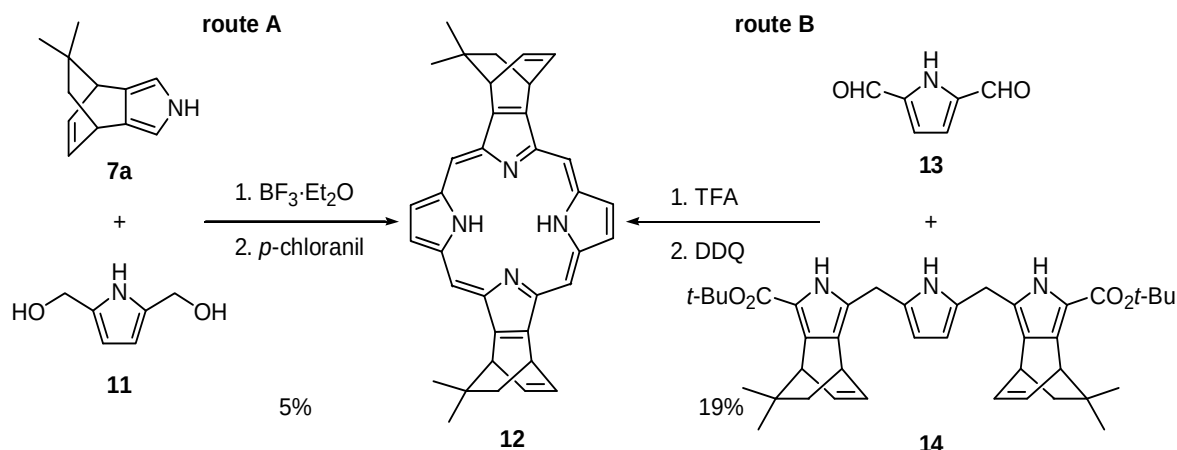
Scheme 4
