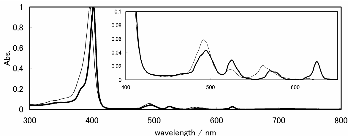
Figure 2. UV-vis spectra of 9 (solid line) and 3 (bold line) in CHCl 3 .
