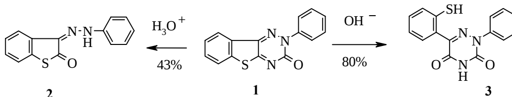
Scheme 1. Acid and basic hydrolysis of 1,2,4-triazine 1
