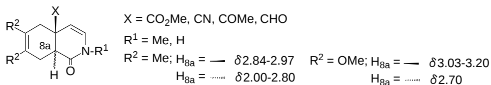
Figure 1. Chemical Shifts ( \delta ) of Isoquinolones 8
