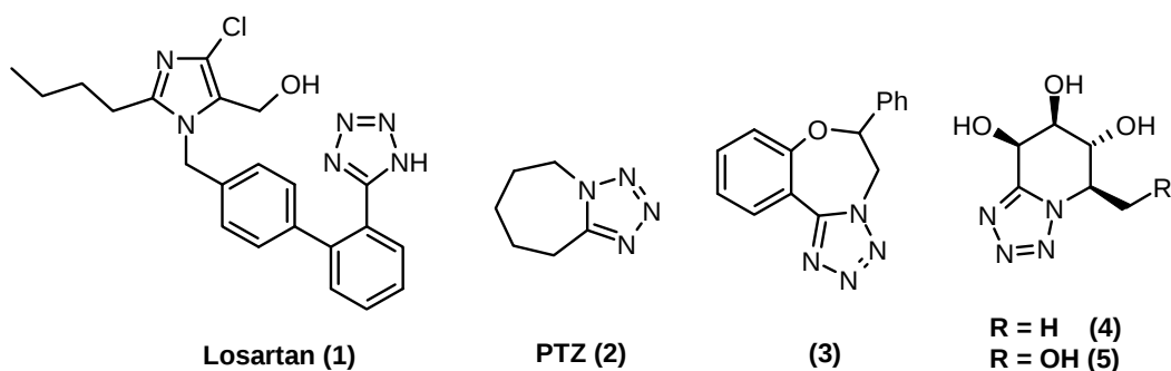
Figure 1. Some annulated benzodiazepines
