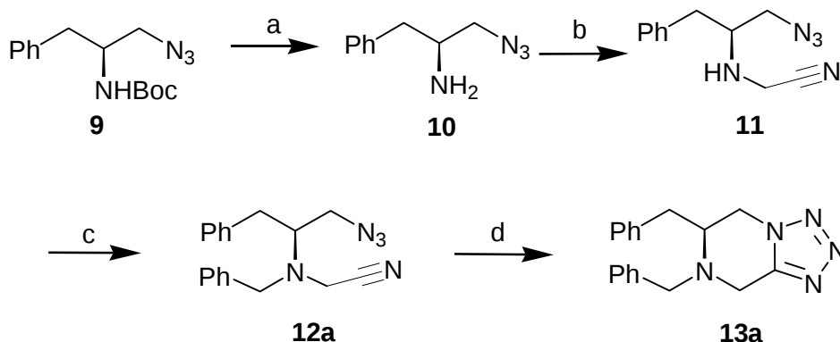
Scheme 2. Reagents and conditions: (a) 4N HCl-EtOAc, 0 °C-rt, 3 h, 88%; (b) K 2 CO 3 , BrCH 2 CN, MeCN, rt, 6 h, 88%; (c) K 2 CO 3 , BnBr, DMF, 80 °C, 6 h, 94%; (d) DMF, 140 °C, 8 h, 90%.
