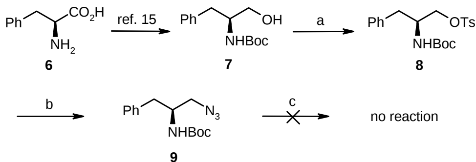
Scheme 1. Reagents and conditions: (a) p -TsCl, Et_3N , CH_2Cl_2 , 0 °C-rt, 8 h, 88%; (b) NaN_3 , DMF, 70 °C, 6 h, 94%; (c) (i) NaH , BrCH_2CN , DMF, 0 °C; (ii) K_2CO_3 , BrCH_2CN , MeCN, rt; (iii) K_2CO_3 , BrCH_2CN , DMF, 80 °C.
