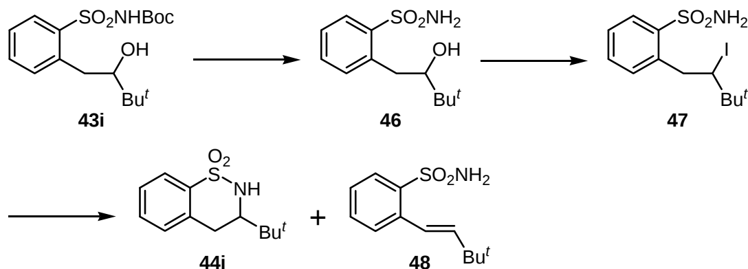
Scheme 18. The Processes of TMSCl-NaI-MeCN Reagent-mediated Cyclization
