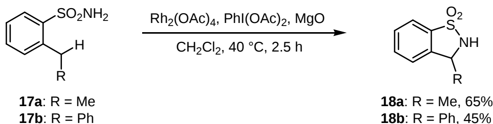
Scheme 5. \text{Rh}^{\text{II}} -catalyzed Intramolecular Sulfonamidation
