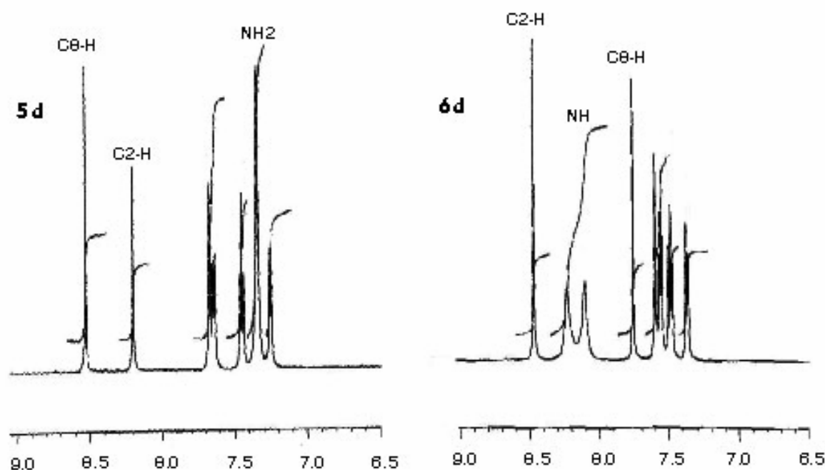
Figure 1: Typical 1 H-NMR spectra of N9- and N3-aryladenines ( 5d and 6d , respectively)
