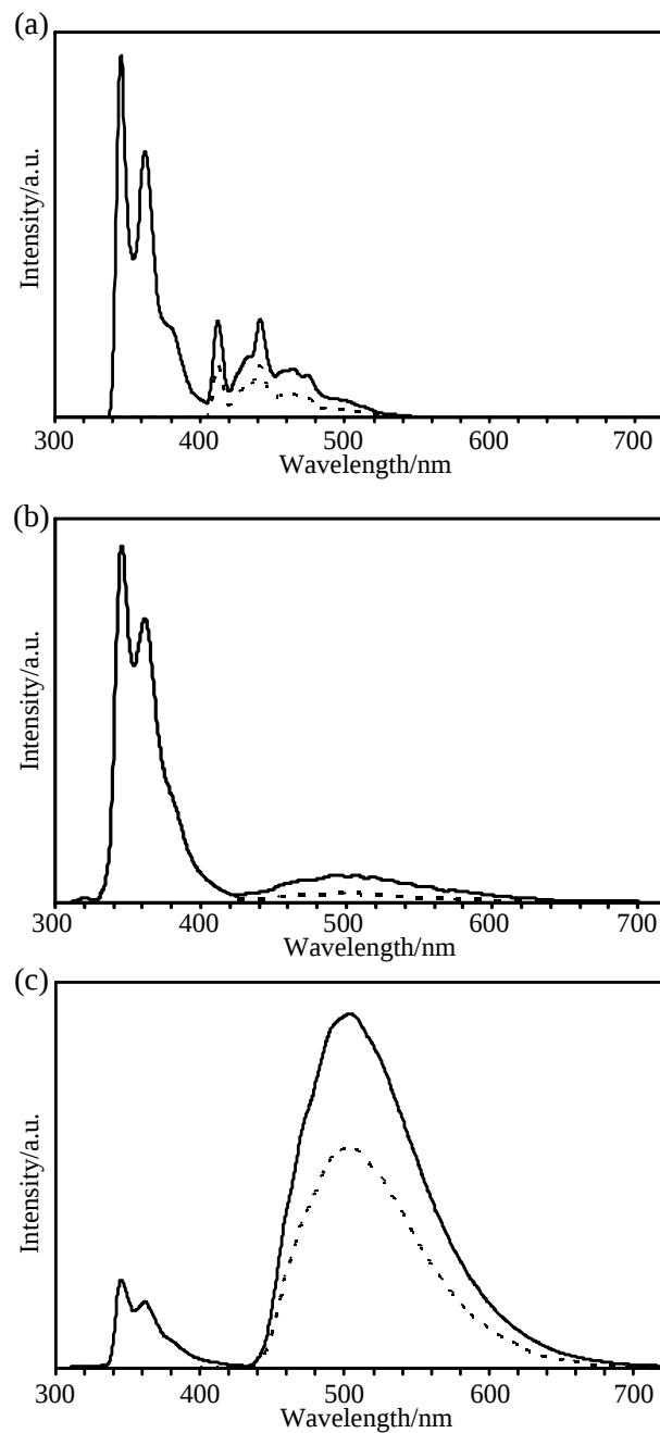
Figure 2. Total emission (solid line) and phosphorescence spectra (dotted line) of (a) 1 , (b) 2 , and (c) 3 in 3-methylpentane at 77 K ( \lambda_{\text{ex}} = 300 \text{ nm} ).
