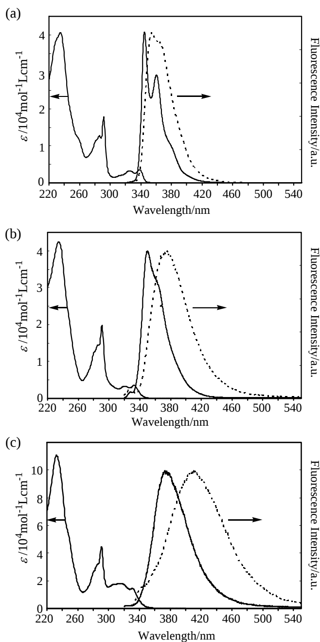
Figure 1. Absorption spectra in cyclohexane and fluorescence spectra ( \lambda_{\text{ex}} = 300 \text{ nm} ) in cyclohexane (solid line) and acetonitrile (dotted line) of (a) 1 , (b) 2 , and (c) 3 at room temperature.
