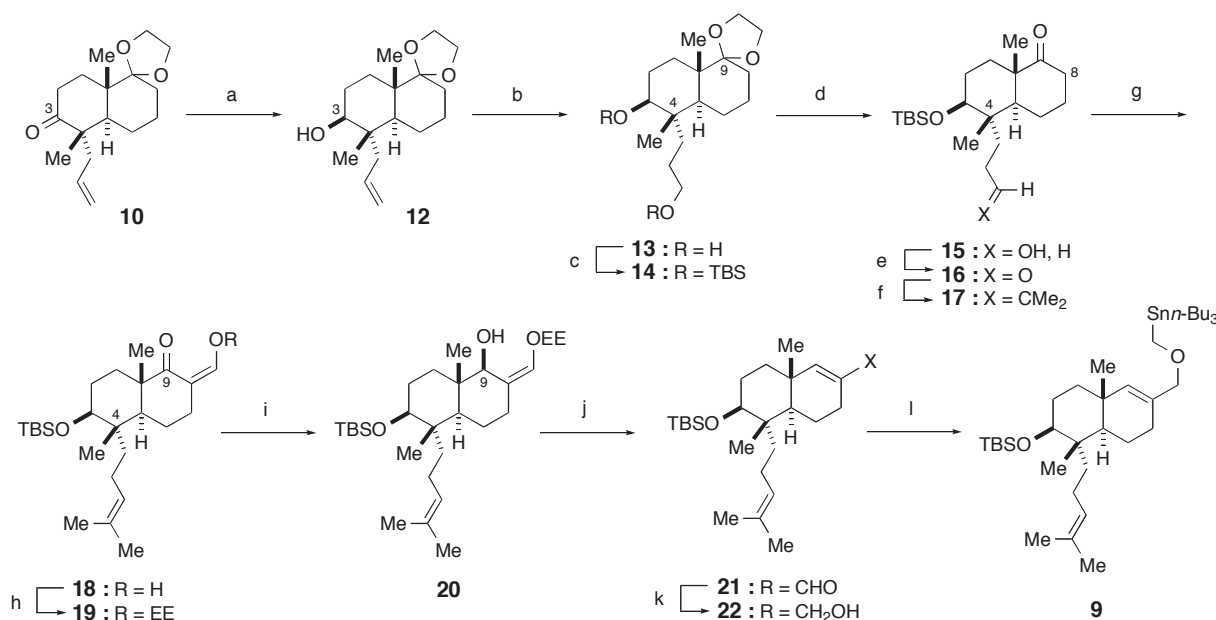
Scheme 2. Synthesis of the key intermediates 9 . Reagents and conditions: (a) LiAlH 4 , Et 2 O, –45 °C to rt, 1.5 h, 98%; (b) BH 3 ·THF, THF, 0 °C to rt, 1 h; 30% aq. H 2 O 2 , 3M NaOH, 0 °C to rt, 1.5 h, 85%; (c) TBSOTf, 2,6-lutidine, CH 2 Cl 2 , 0 °C, 30 min, quant.; (d) AcOH/THF/H 2 O (3:1:1), 50 °C, 4 h, 90%; (e) Dess–Martin periodinane, CH 2 Cl 2 , rt, 96%; (f) Ph 3 PCHMe 2 I, n -BuLi, THF, 0 °C, 1 h, 86%; (g) ethyl formate, NaH, THF, 0° to rt, 1 h, quant.; (h) ethyl vinyl ether, PPTS, rt, 4 h, 91%; (i) NaBH 4 , EtOH, 0 °C to rt, 2 h, 92%; (j) MsCl, Et 3 N, CH 2 Cl 2 , 0 °C, 30 min, 94% (k) NaBH 4 , EtOH, 0 °C to rt, 30 min, quant.; (l) n -Bu 3 SnCH 2 I, KH, 18-crown-6, THF, 0 °C to rt, 1 h, 98%
