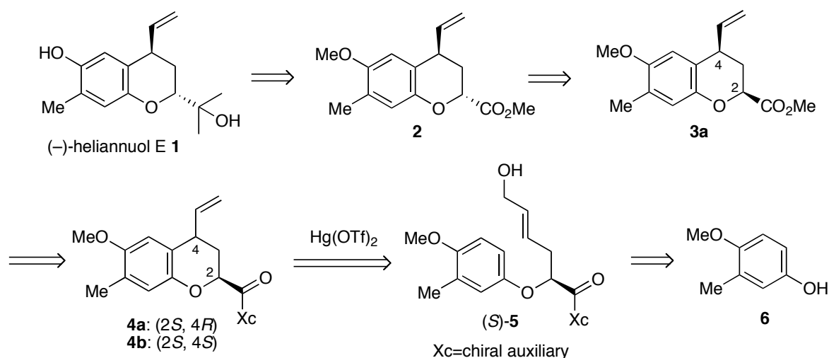
Scheme 1. Retrosynthetic Analysis
