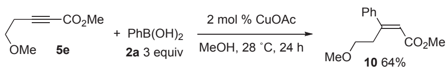
Scheme 8. Hydroarylation of 5-(methoxy)-2-pentyne-1-carboxylate methyl ester 5e
