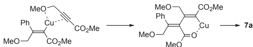
Scheme 4. Proposed pathway to 2:1 adduct 7a
