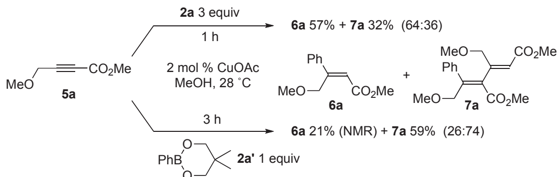
Scheme 3. Hydroarylation of 4-methoxy-2-butynoate 5a
