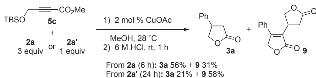
Scheme 6. Hydroarylation/lactonization of 4-( tert -butyldimethylsilyloxy)-2-butyne-1-carboxylate methyl ester 5c
