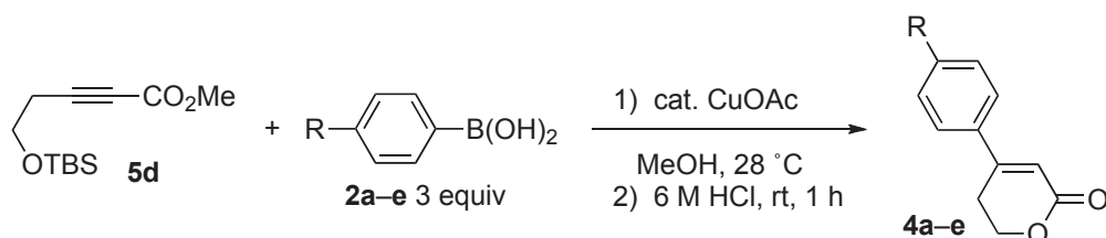
Scheme 7. Hydroarylation/lactonization of 5-( tert -butyldimethylsilyloxy)-2-pentyne-1-carboxylate methyl ester 5d
