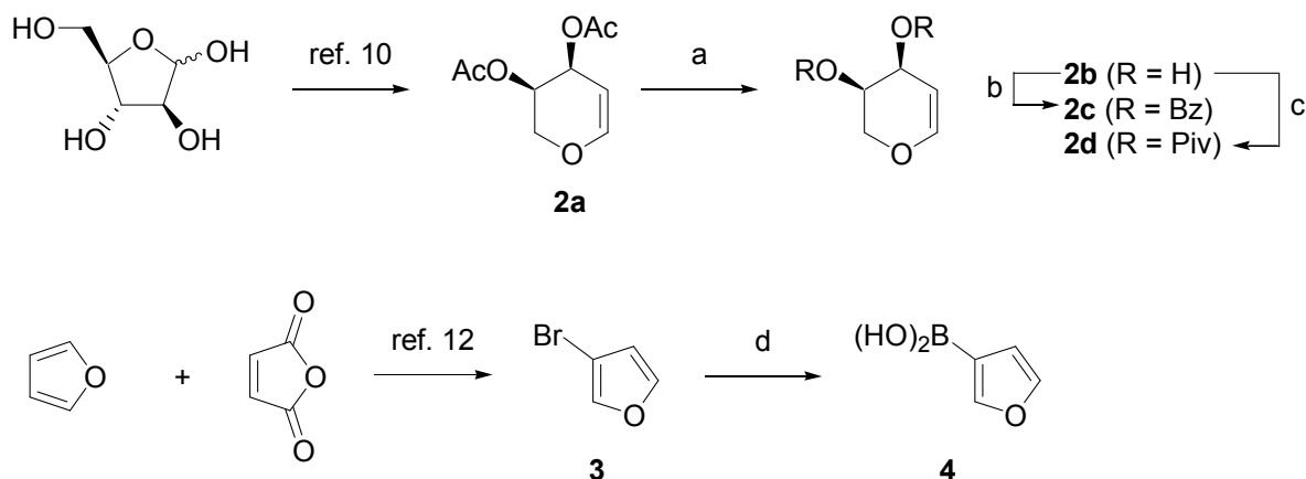
Scheme 2. Synthesis of substrates for Pd-mediated C-glycosidation. Reagents and conditions: (a) K_2CO_3 , MeOH, rt, 98%; (b) BzCl, pyridine, 0 °C→rt, quant.; (c) PivCl, Et_3N , CH_2Cl_2 , 0 °C→rt, 9%; (d) n-BuLi ; (i-PrO)_3B ; aq. HCl, 67%.
