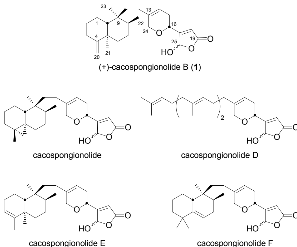
Figure 1. Structures of cacospongionolide family
