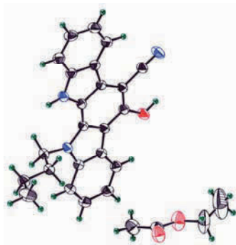
Figure 1. ORTEP Drawing of 9a ( R=0.049 )
