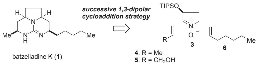
Scheme 1. Synthetic plan for batzelladine K (1).
