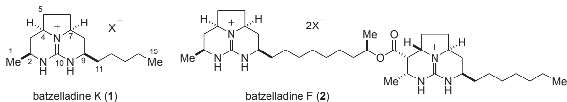
Figure 1. Structures of batzelladines K (1) and F (2).
