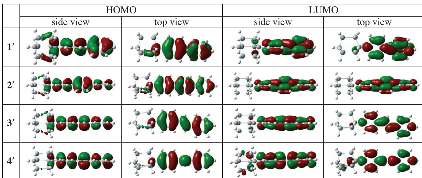
Figure 14. HOMO and LUMO orbitals of 1' – 4' (HF/6-31G(d)//B3LYP/6-31G(d) level).
