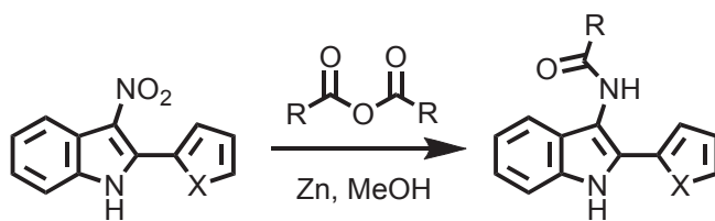
Scheme 4. Mild reductive-acylation
