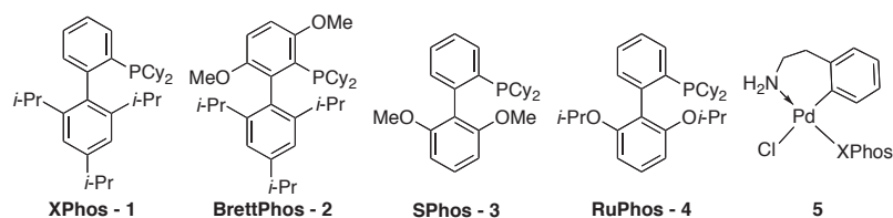
Figure 1: Biaryl-monophosphine Ligands
