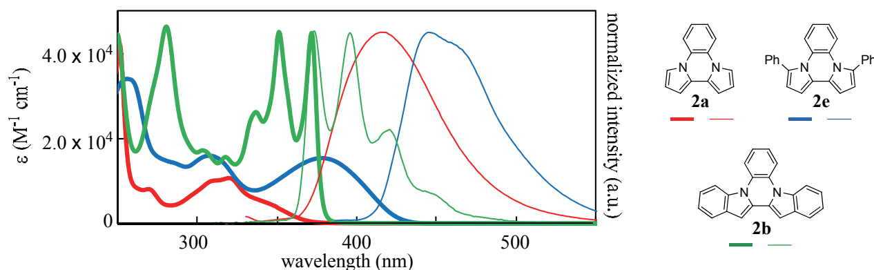
Figure 1. UV-VIS Absorption (bold line; 3.0 \times 10^{-5} M in THF) and fluorescence (narrow line; 3.0 \times 10^{-7} M in THF) spectra of 2a (red), 2e (blue), and 2b (green).
