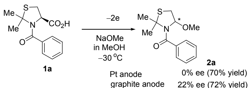
Scheme 2. Electrochemical oxidation of thiazolidine derivative 1a
