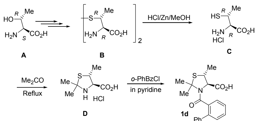
Scheme 8. Preparation of cysteine derivative 1d
