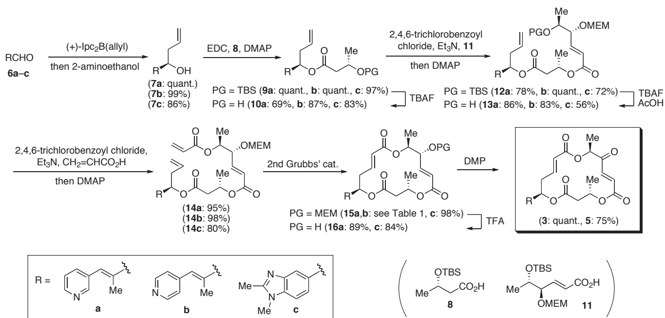
Scheme 1. Synthesis of Macrophelide Analogues 3 and 5
