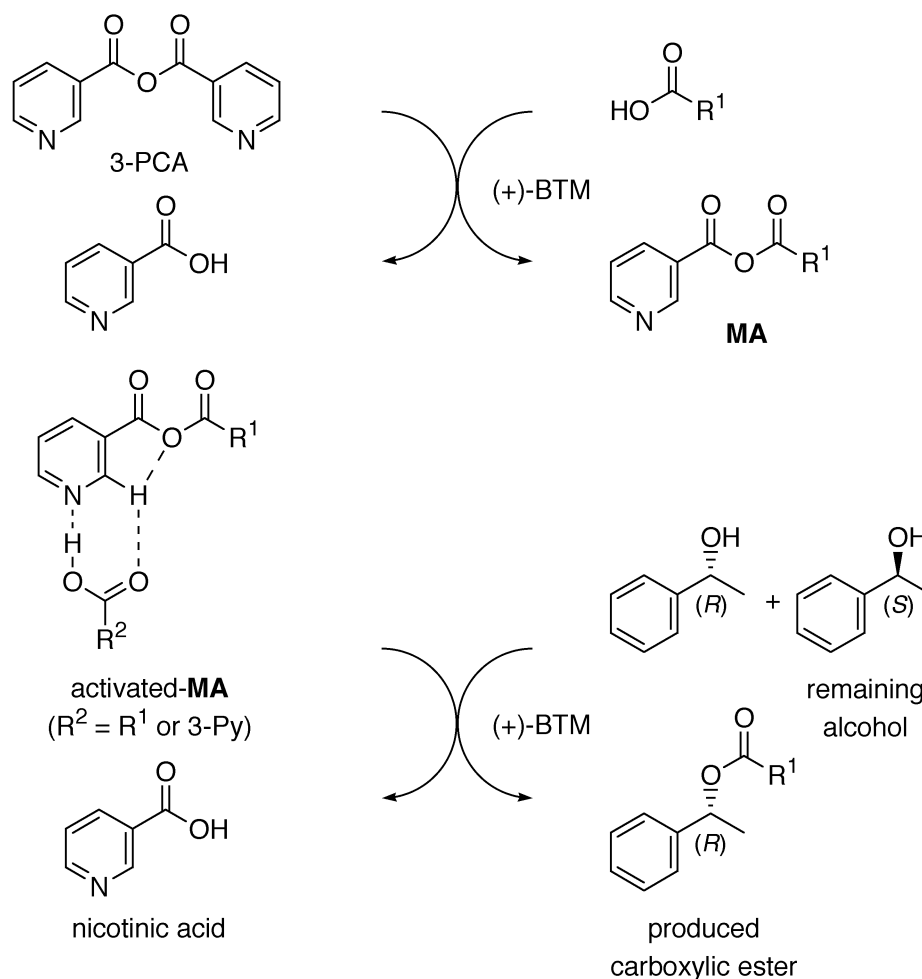
Scheme 3. Proposed Reaction Pathway of the Kinetic Resolution
