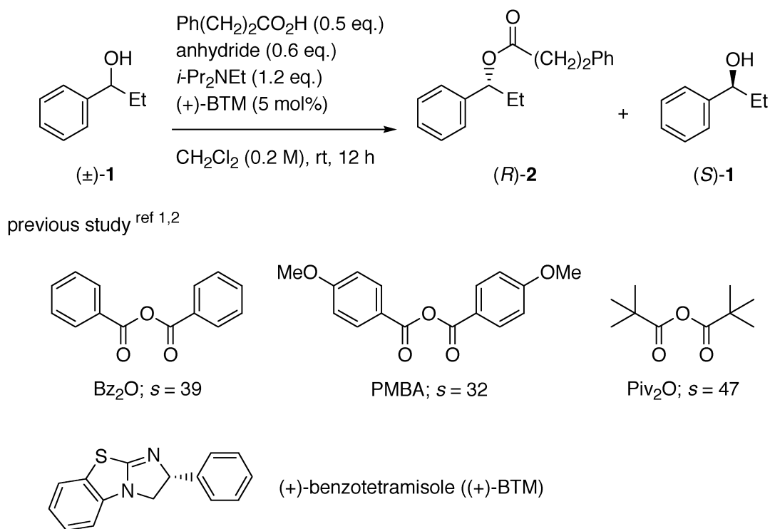
Scheme 1. Kinetic Resolution of (±)-1 Using Bz 2 O, PMBA, and Piv 2 O (Our Previous Study)
