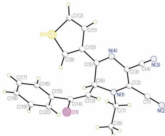
Figure 3. X-Ray crystal structure of compound ( E-4b )
