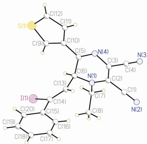
Figure 4. X-Ray crystal structure of compound ( Z-4b )
