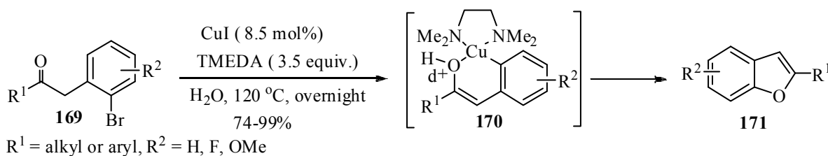
Scheme 53. CuI-Catalyzed cyclization of 2-haloaromatic ketones to substituted benzo[ b ]furans
