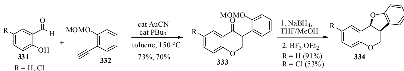
Scheme 99. Au(I)-Catalyzed synthesis of ( \pm )-pterocarpan
