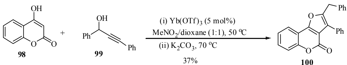
Scheme 31. \text{Yb} -Catalyzed synthesis of furocoumarin
