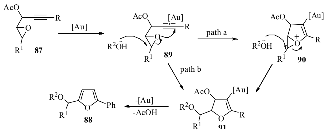
Scheme 29. Mechanism of cycloisomerization /alkoxylation of alkynyloxiranes
