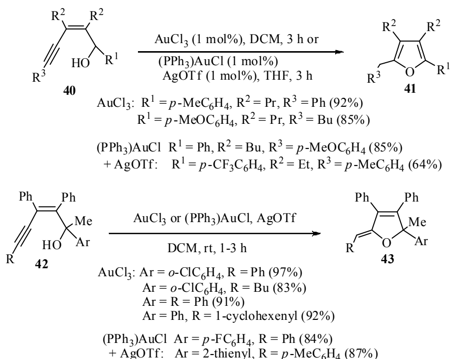
Scheme 13. Au-Catalyzed cycloisomerization of sec - and tert -alcohols to tetrasubstituted furans
