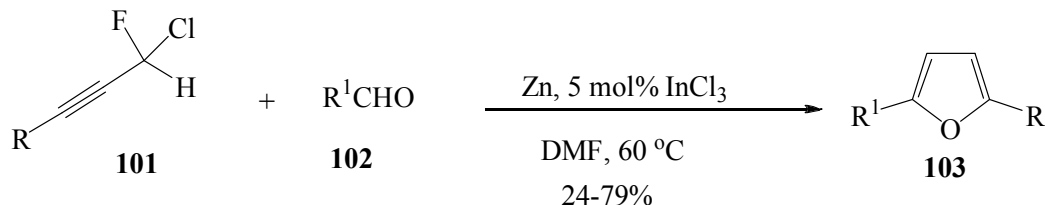
Scheme 32. \text{InCl}_3 -Catalyzed synthesis of 2,5-disubstituted furans from fluoropropargyl chloride
