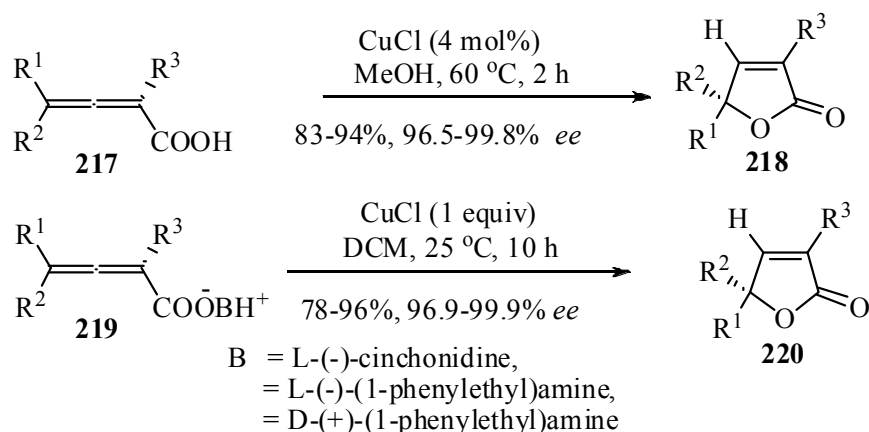
Scheme 69. Cu-Catalyzed cyclization of 2,3-allenoic acids to 2(5 H )-furanones
