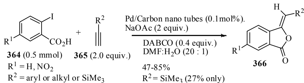
Scheme 108. Pd/carbon Nanotubes-Catalyzed synthesis of phthalides
