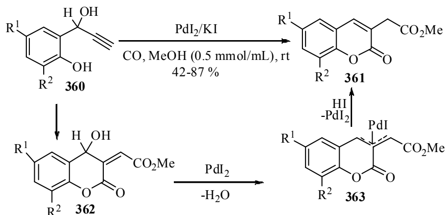
Scheme 107. PdI 2 -catalyzed synthesis of 3-[(methoxycarbonyl)methyl]coumarins
