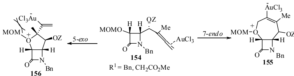
Scheme 49. Mode of regioselectivity cyclization
