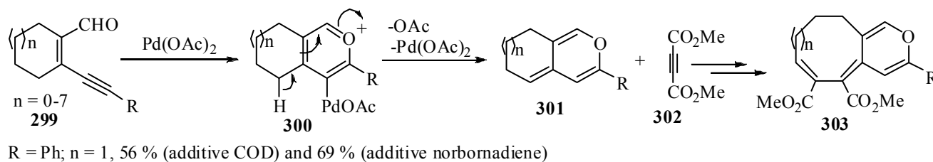
Scheme 90. \text{Pd}(\text{OAc})_2 -Catalyzed synthesis of pyran derivatives fused with medium to large rings
