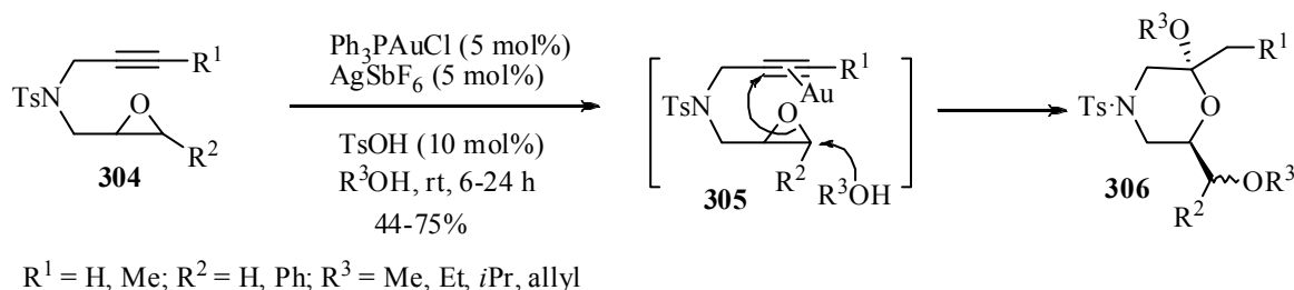
Scheme 91. \text{Au}(\text{I}) -Catalyzed ring-opening of epoxides to 2,6- trans -substituted morpholine
