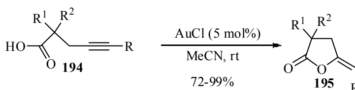
Scheme 61. Au(I)-Catalyzed cyclization of acetylenic acids to \gamma -lactones
