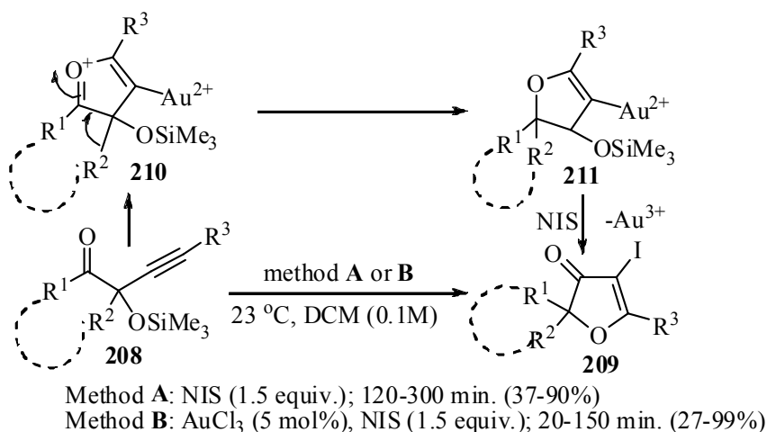
Scheme 66. Tandem cyclization/1,2-migration of 2-alkynyl-2-siloxy carbonyls to 3(2 H )-furanones
