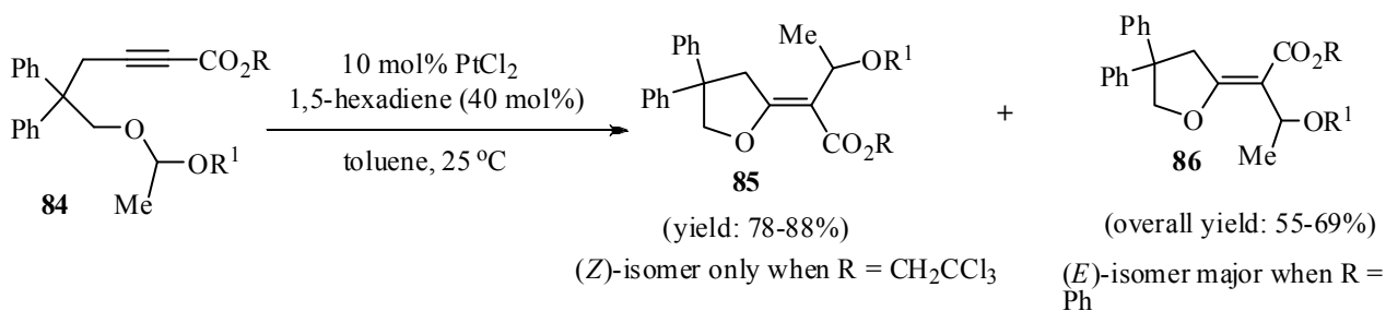
Scheme 27. Pt-Catalyzed stereoselective synthesis of dihydrofuran derivatives
