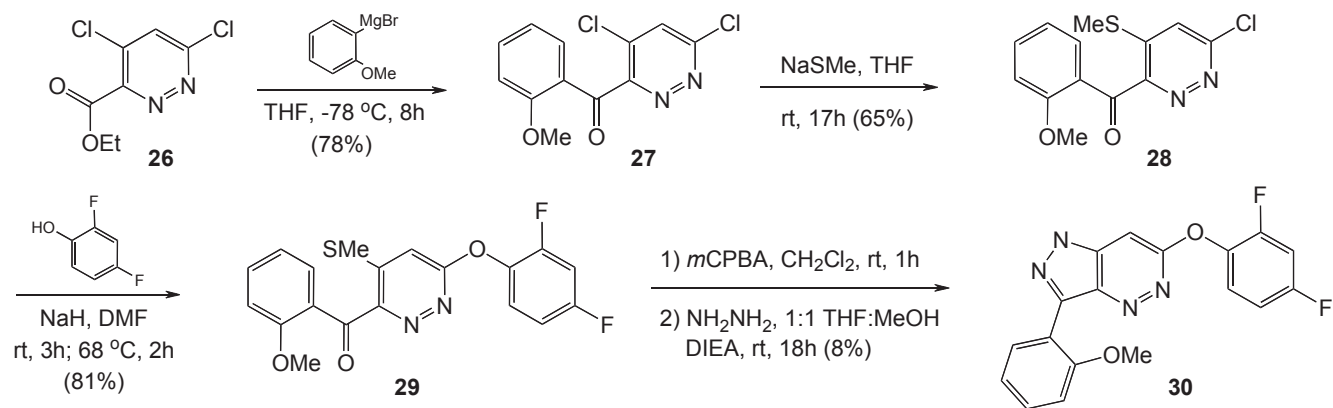
Scheme 5
