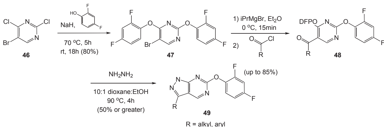
Scheme 9
