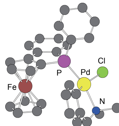
Fig. 1 X-Ray structure of 8
