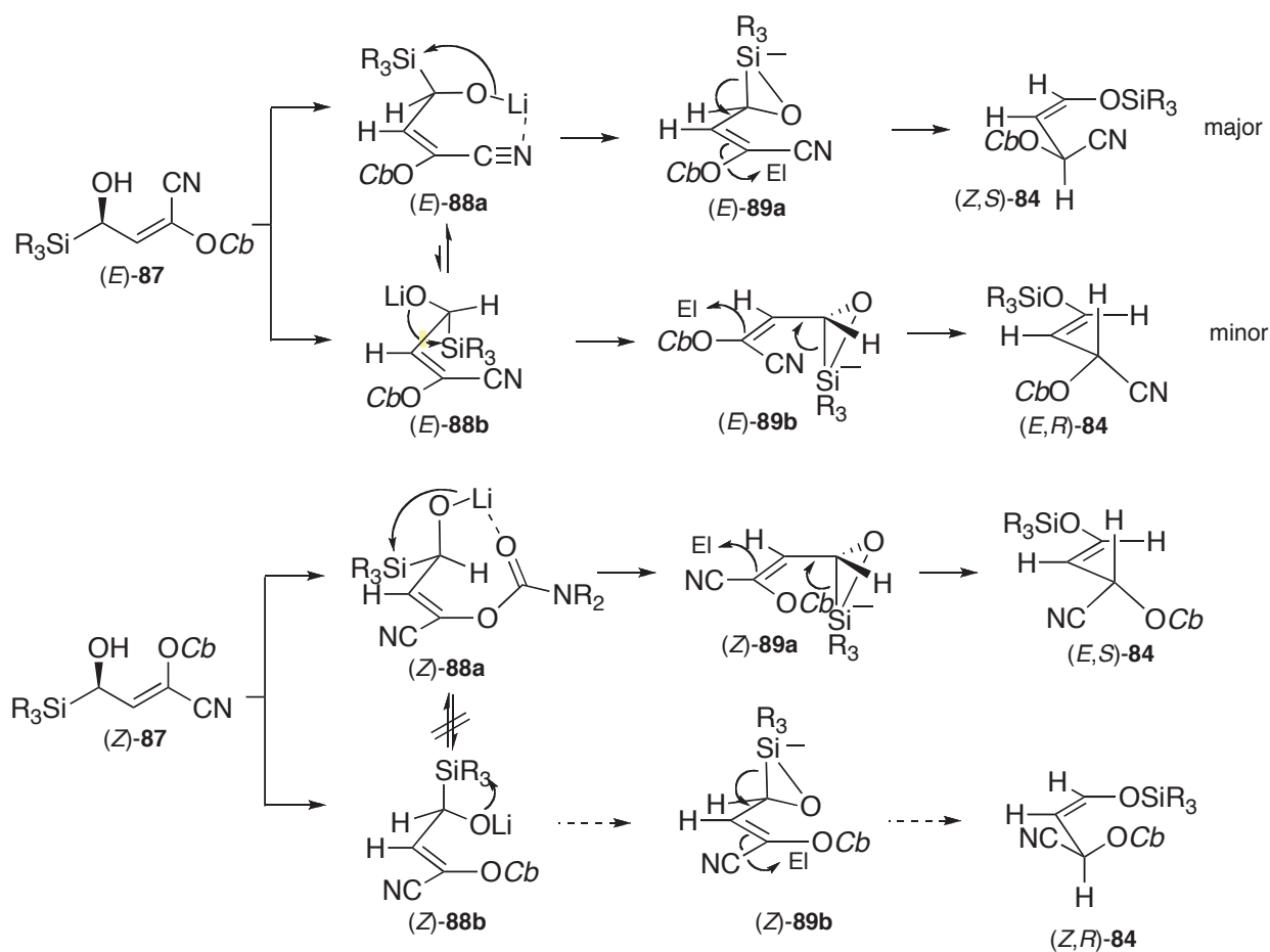
Scheme 21
