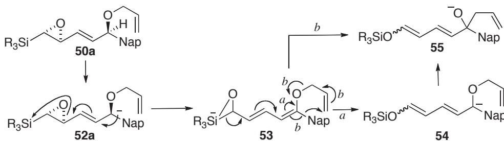
Scheme 14
