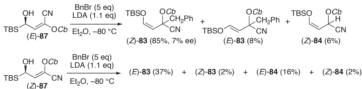
Scheme 19
