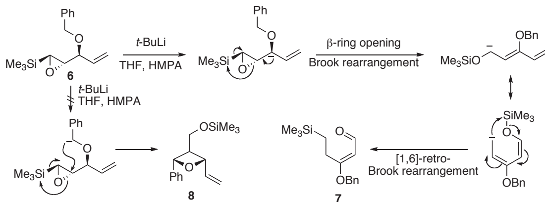
Scheme 4
